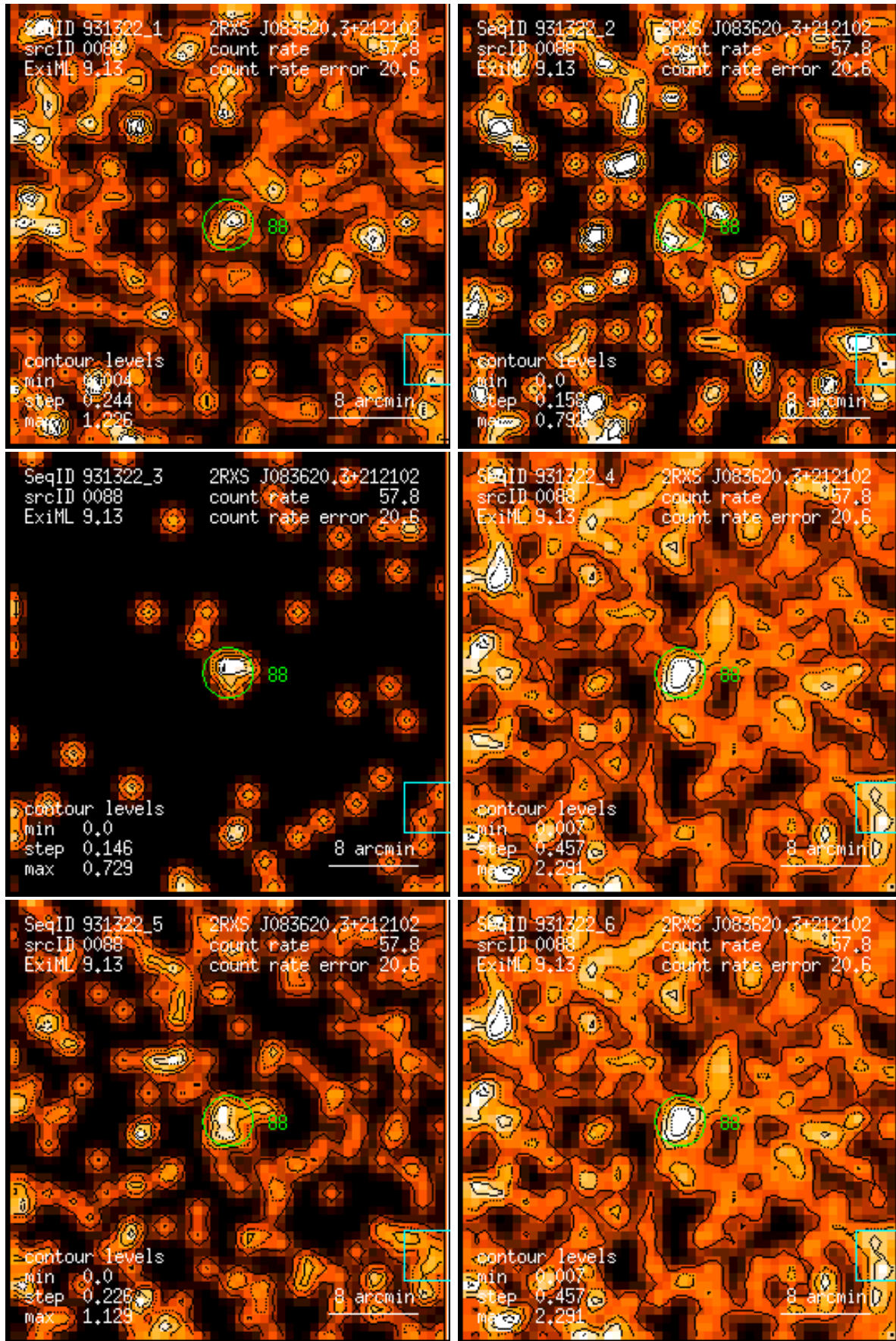
Figure 88: RASS 931322: detection 0088: band rate images, Gaussian filter: (1) PSPC channels 11 – 41, (2) 52 – 90, (3) 91 – 201, (4) 11 – 235, (5) 52 – 201, (6) 11 – 201. Broad band rates in counts/ks. Band rate contour levels in counts/ks/arcmin 2 .
