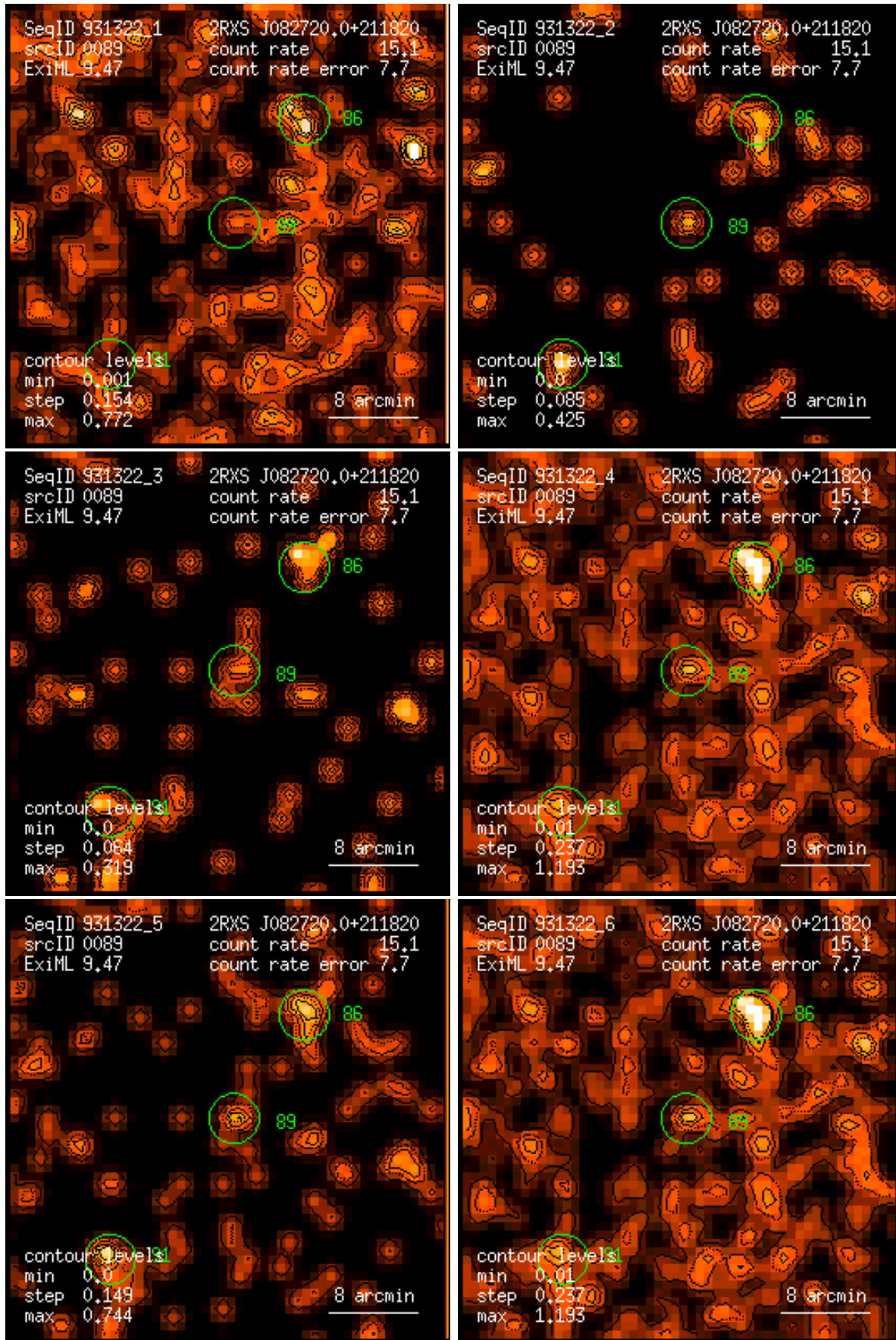
Figure 89: RASS 931322: detection 0089: band rate images, Gaussian filter: (1) PSPC channels 11 – 41, (2) 52 – 90, (3) 91 – 201, (4) 11 – 235, (5) 52 – 201, (6) 11 – 201. Broad band rates in counts/ks. Band rate contour levels in counts/ks/arcmin 2 .
