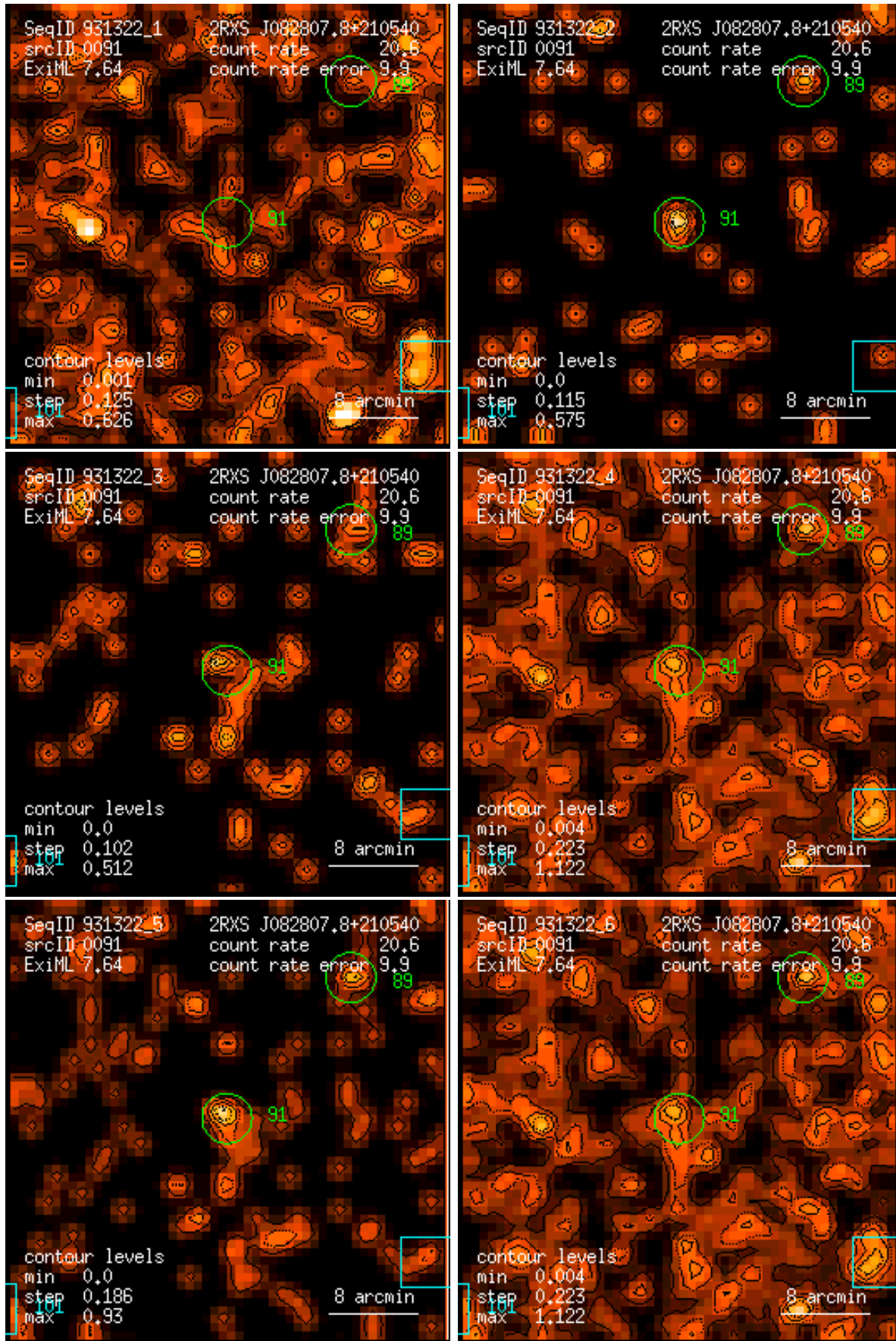
Figure 91: RASS 931322: detection 0091: band rate images, Gaussian filter: (1) PSPC channels 11 – 41, (2) 52 – 90, (3) 91 – 201, (4) 11 – 235, (5) 52 – 201, (6) 11 – 201. Broad band rates in counts/ks. Band rate contour levels in counts/ks/arcmin 2 .
