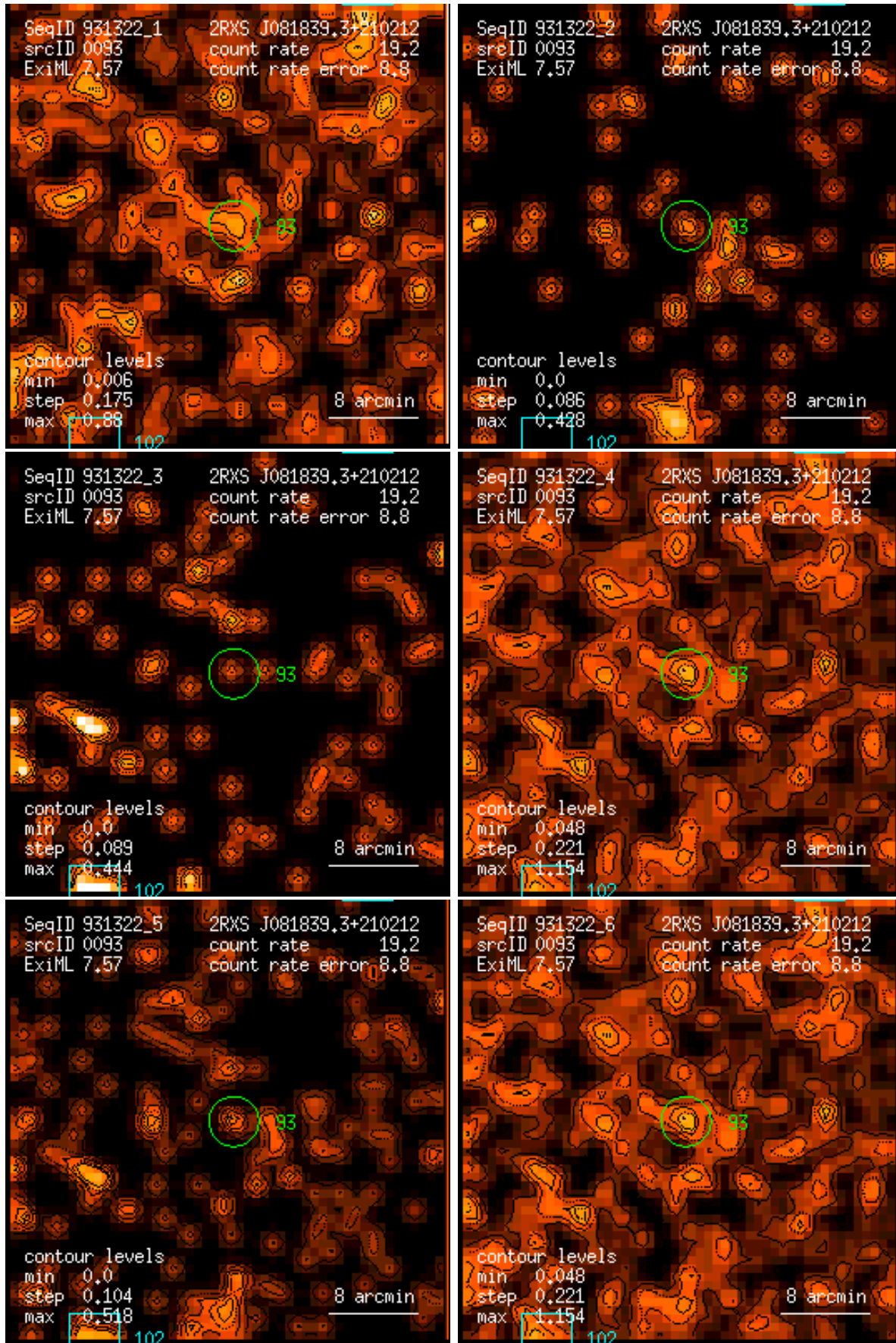
Figure 93: RASS 931322: detection 0093: band rate images, Gaussian filter: (1) PSPC channels 11 – 41, (2) 52 – 90, (3) 91 – 201, (4) 11 – 235, (5) 52 – 201, (6) 11 – 201. Broad band rates in counts/ks. Band rate contour levels in counts/ks/arcmin 2 .
