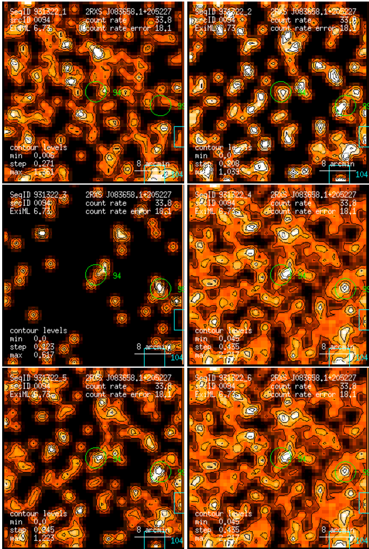
Figure 94: RASS 931322: detection 0094: band rate images, Gaussian filter: (1) PSPC channels 11 – 41, (2) 52 – 90, (3) 91 – 201, (4) 11 – 235, (5) 52 – 201, (6) 11 – 201. Broad band rates in counts/ks. Band rate contour levels in counts/ks/arcmin 2 .
