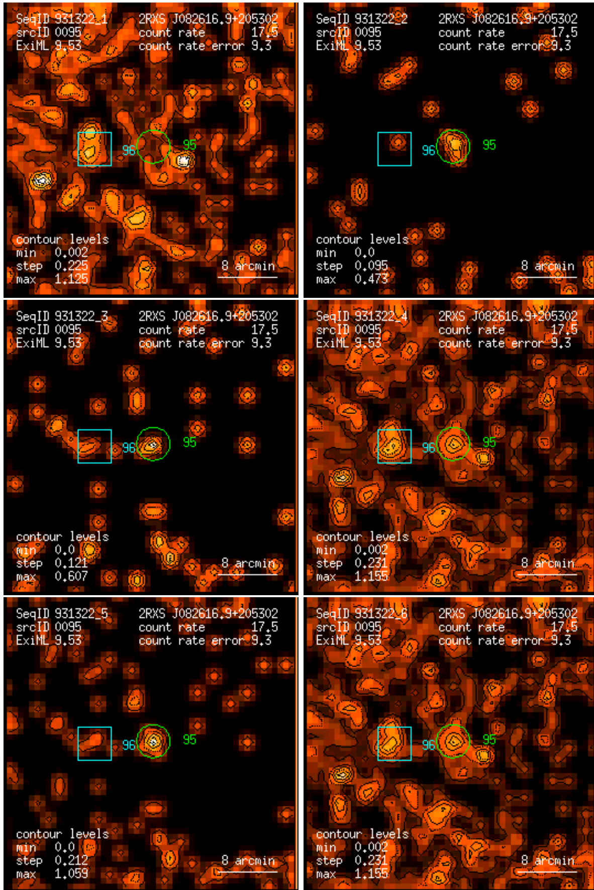
Figure 95: RASS 931322: detection 0095: band rate images, Gaussian filter: (1) PSPC channels 11 – 41, (2) 52 – 90, (3) 91 – 201, (4) 11 – 235, (5) 52 – 201, (6) 11 – 201. Broad band rates in counts/ks. Band rate contour levels in counts/ks/arcmin 2 .
