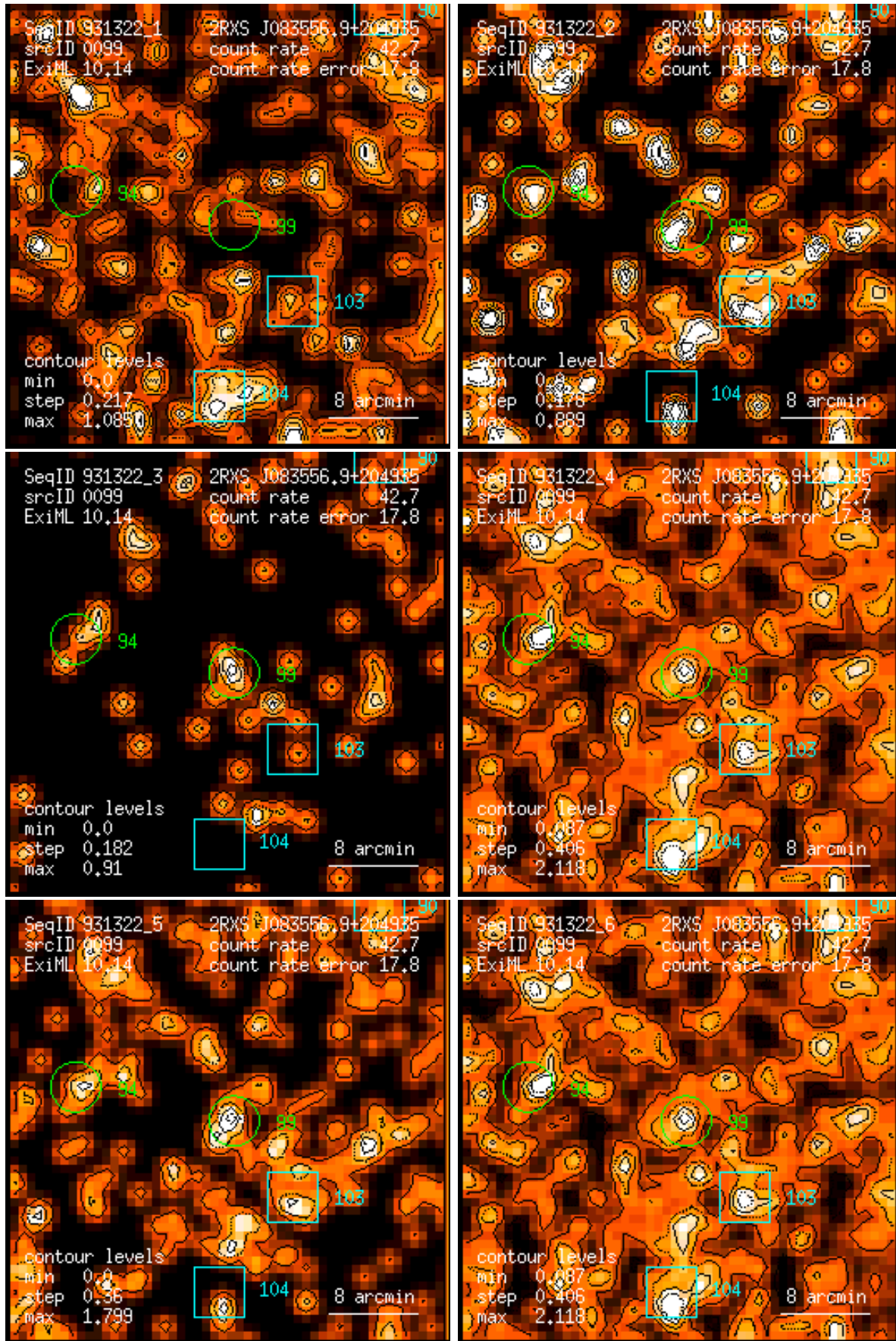
Figure 99: RASS 931322: detection 0099: band rate images, Gaussian filter: (1) PSPC channels 11 – 41, (2) 52 – 90, (3) 91 – 201, (4) 11 – 235, (5) 52 – 201, (6) 11 – 201. Broad band rates in counts/ks. Band rate contour levels in counts/ks/arcmin 2 .
