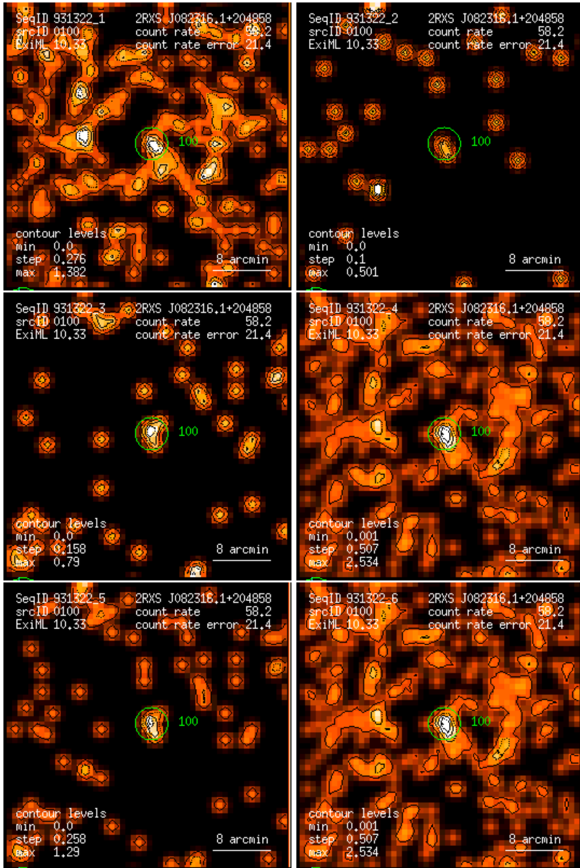
Figure 100: RASS 931322: detection 0100: band rate images, Gaussian filter: (1) PSPC channels 11 – 41, (2) 52 – 90, (3) 91 – 201, (4) 11 – 235, (5) 52 – 201, (6) 11 – 201. Broad band rates in counts/ks. Band rate contour levels in counts/ks/arcmin 2 .
