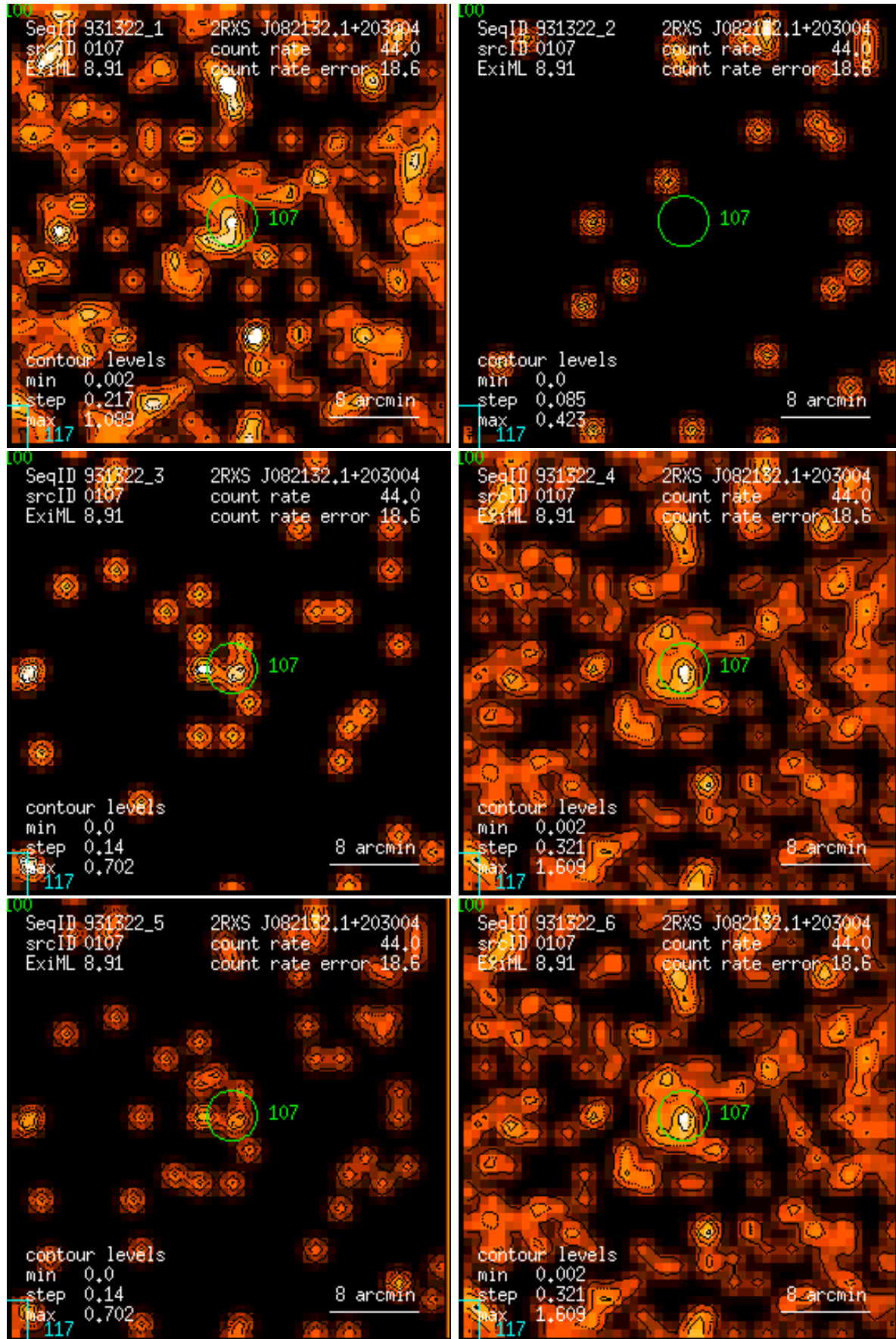
Figure 107: RASS 931322: detection 0107: band rate images, Gaussian filter: (1) PSPC channels 11 – 41, (2) 52 – 90, (3) 91 – 201, (4) 11 – 235, (5) 52 – 201, (6) 11 – 201. Broad band rates in counts/ks. Band rate contour levels in counts/ks/arcmin 2 .
