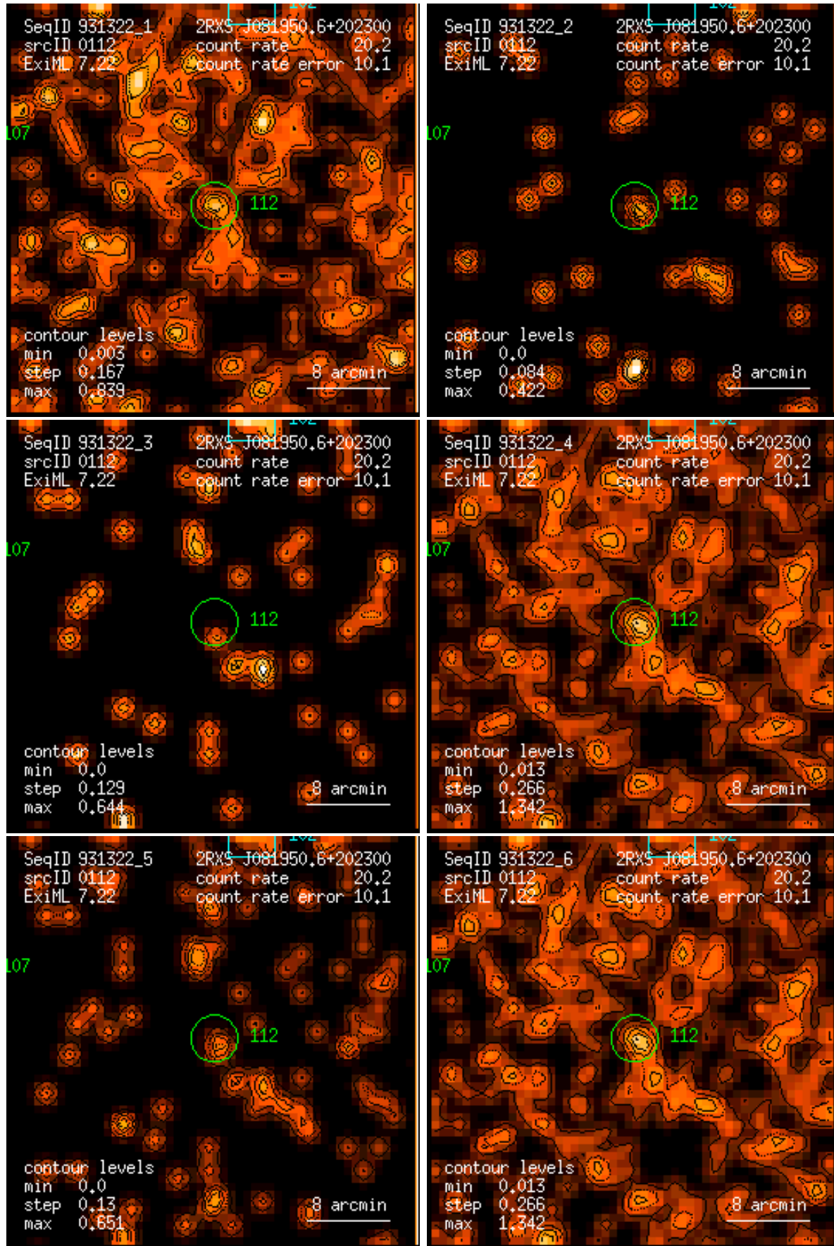
Figure 112: RASS 931322: detection 0112: band rate images, Gaussian filter: (1) PSPC channels 11 – 41, (2) 52 – 90, (3) 91 – 201, (4) 11 – 235, (5) 52 – 201, (6) 11 – 201. Broad band rates in counts/ks. Band rate contour levels in counts/ks/arcmin 2 .
