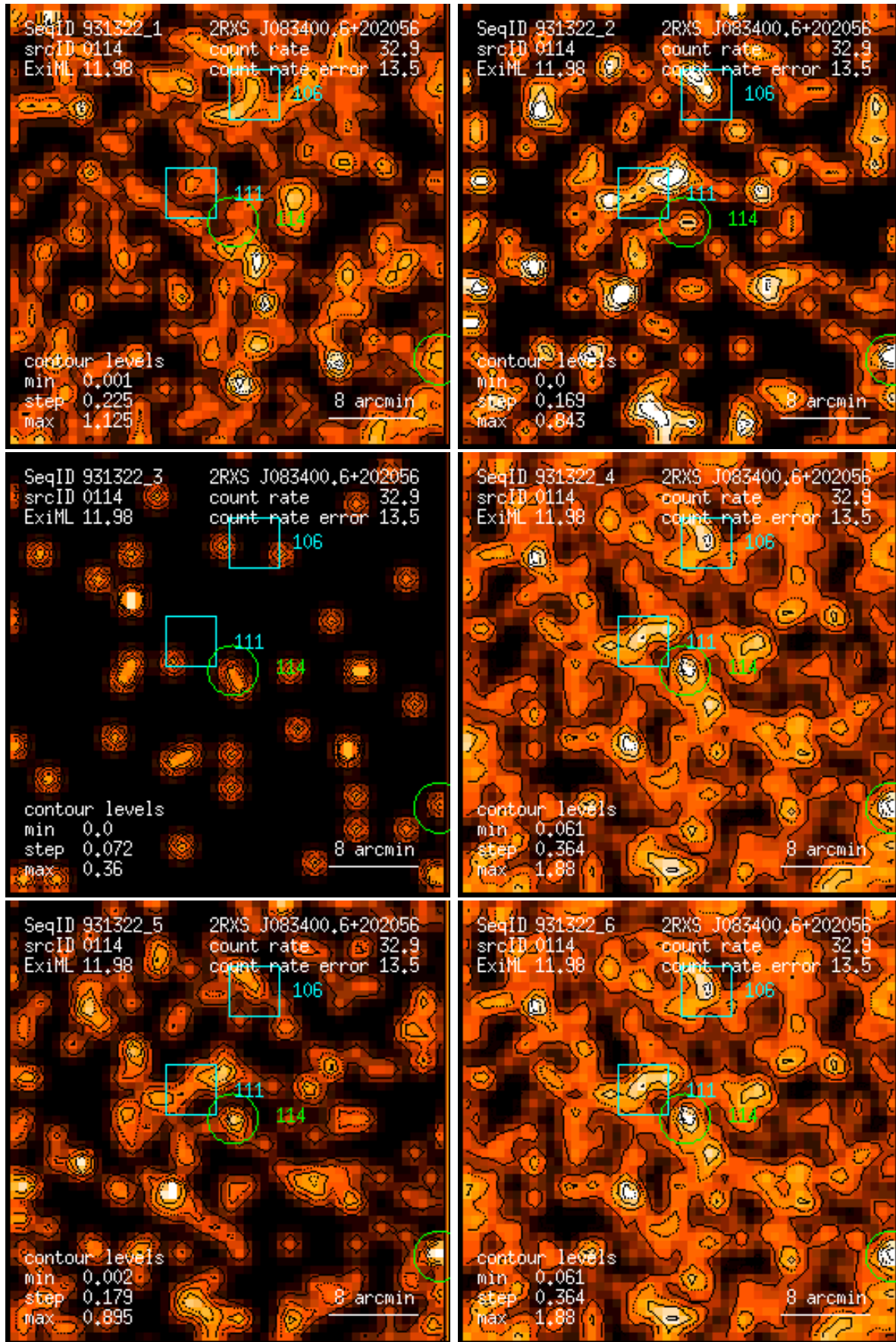
Figure 114: RASS 931322: detection 0114: band rate images, Gaussian filter: (1) PSPC channels 11 – 41, (2) 52 – 90, (3) 91 – 201, (4) 11 – 235, (5) 52 – 201, (6) 11 – 201. Broad band rates in counts/ks. Band rate contour levels in counts/ks/arcmin 2 .
