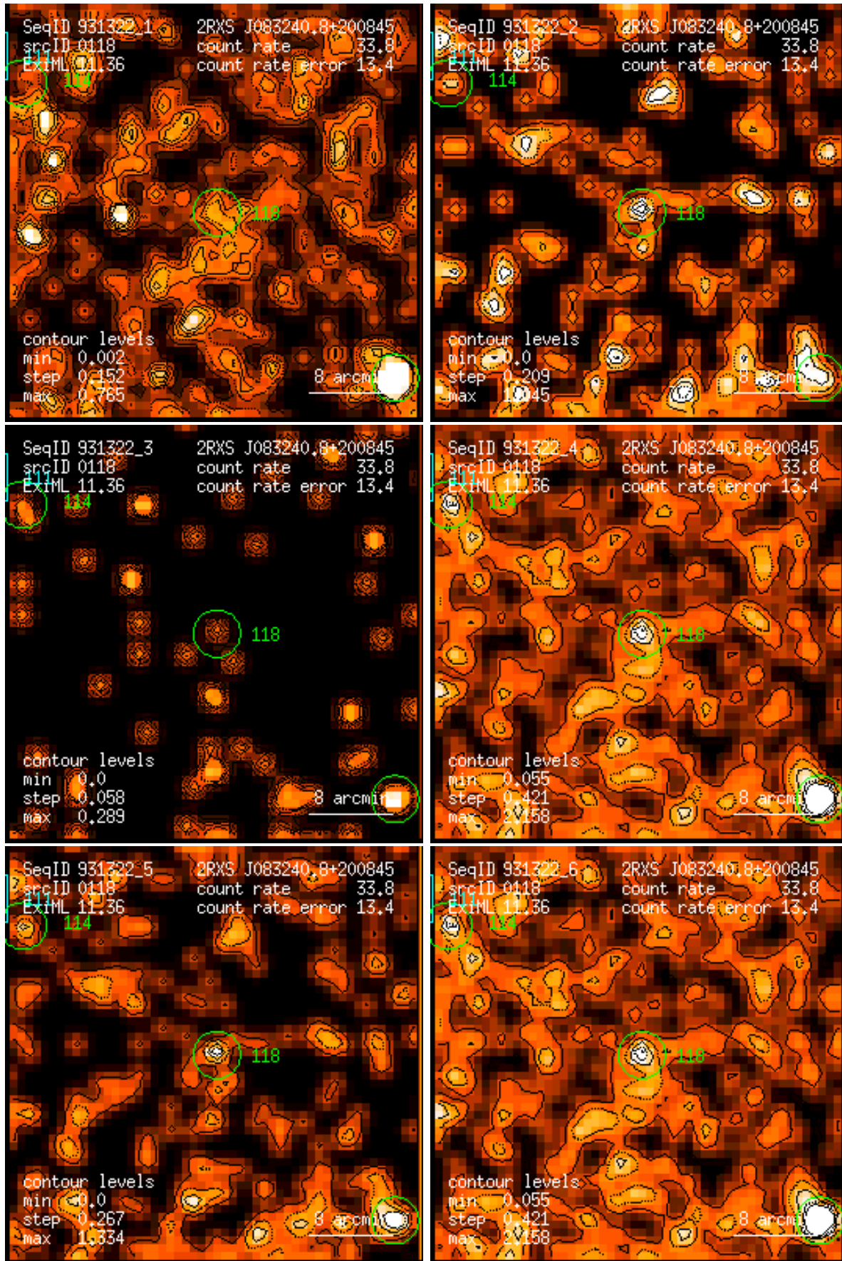
Figure 118: RASS 931322: detection 0118: band rate images, Gaussian filter: (1) PSPC channels 11 – 41, (2) 52 – 90, (3) 91 – 201, (4) 11 – 235, (5) 52 – 201, (6) 11 – 201. Broad band rates in counts/ks. Band rate contour levels in counts/ks/arcmin 2 .
