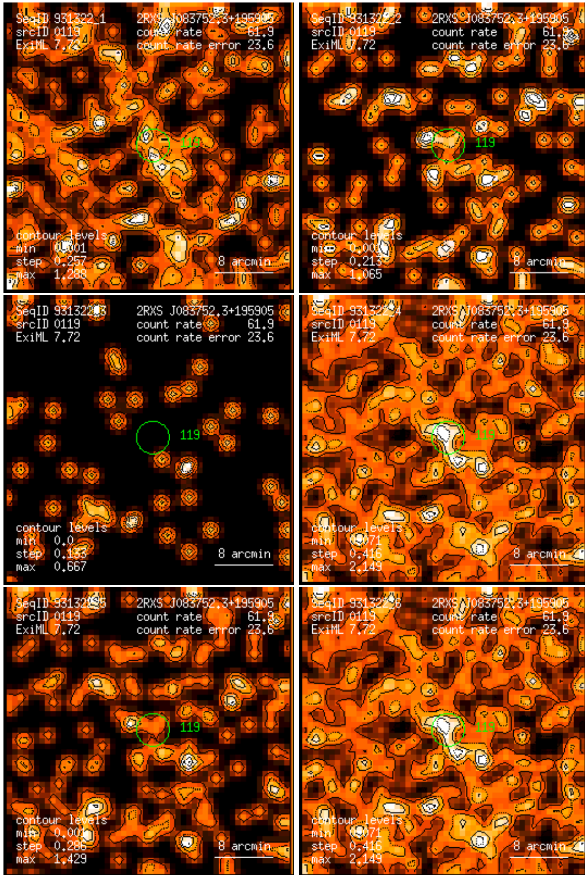
Figure 119: RASS 931322: detection 0119: band rate images, Gaussian filter: (1) PSPC channels 11 – 41, (2) 52 – 90, (3) 91 – 201, (4) 11 – 235, (5) 52 – 201, (6) 11 – 201. Broad band rates in counts/ks. Band rate contour levels in counts/ks/arcmin 2 .
