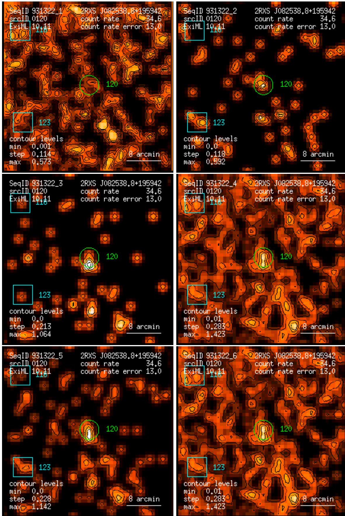
Figure 120: RASS 931322: detection 0120: band rate images, Gaussian filter: (1) PSPC channels 11 – 41, (2) 52 – 90, (3) 91 – 201, (4) 11 – 235, (5) 52 – 201, (6) 11 – 201. Broad band rates in counts/ks. Band rate contour levels in counts/ks/arcmin 2 .
