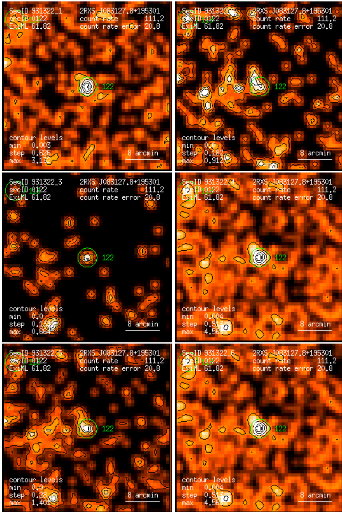
Figure 122: RASS 931322: detection 0122: band rate images, Gaussian filter: (1) PSPC channels 11 – 41, (2) 52 – 90, (3) 91 – 201, (4) 11 – 235, (5) 52 – 201, (6) 11 – 201. Broad band rates in counts/ks. Band rate contour levels in counts/ks/arcmin 2 .
