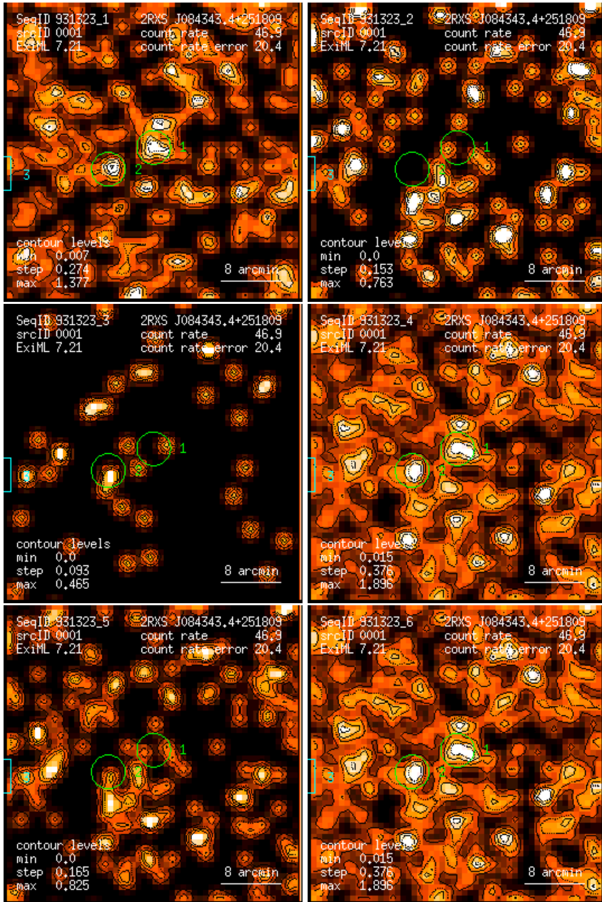
Figure 1: RASS 931323: detection 0001: band rate images, Gaussian filter: (1) PSPC channels 11 – 41, (2) 52 – 90, (3) 91 – 201, (4) 11 – 235, (5) 52 – 201, (6) 11 – 201. Broad band rates in counts/ks. Band rate contour levels in counts/ks/arcmin 2 .
