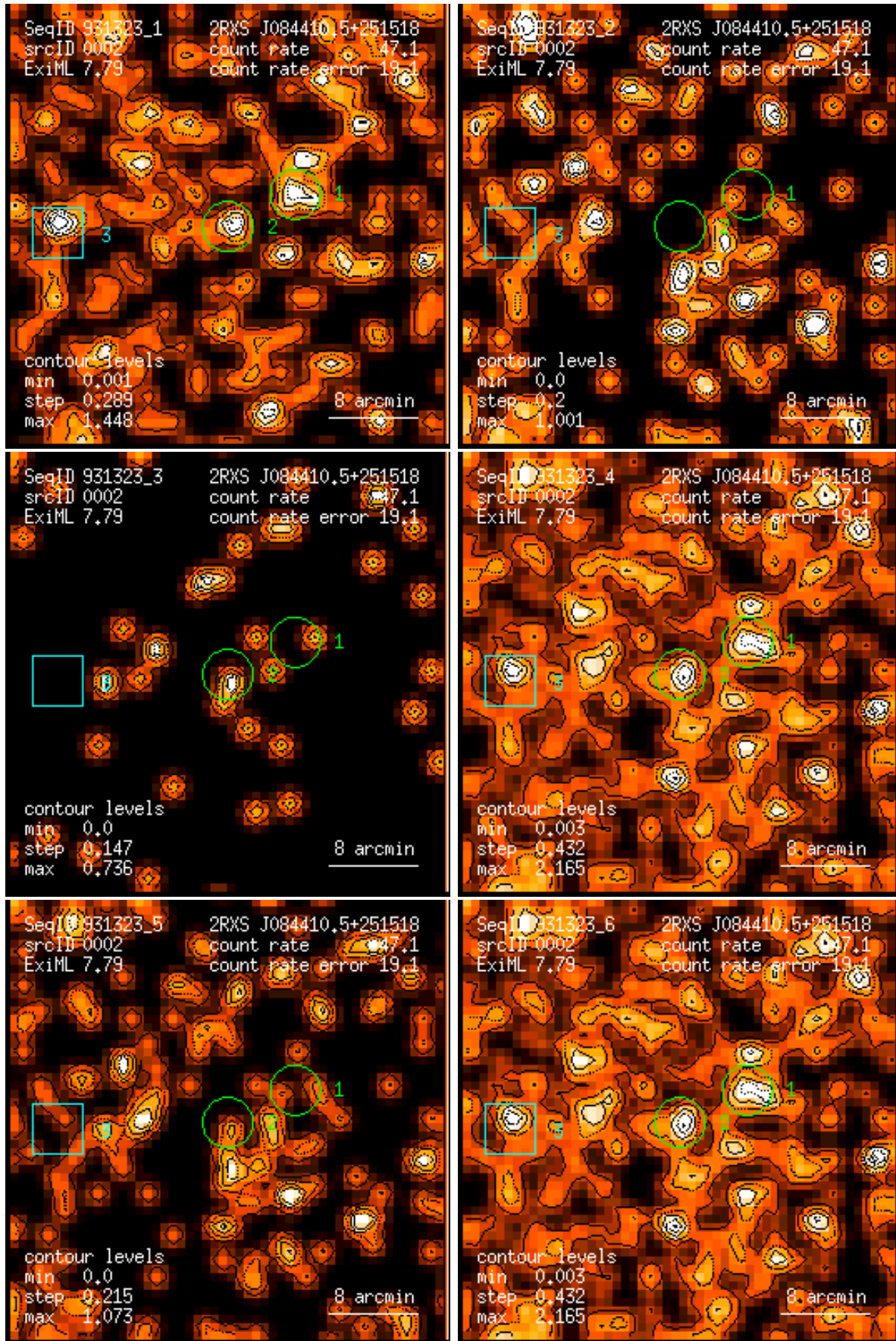
Figure 2: RASS 931323: detection 0002: band rate images, Gaussian filter: (1) PSPC channels 11 – 41, (2) 52 – 90, (3) 91 – 201, (4) 11 – 235, (5) 52 – 201, (6) 11 – 201. Broad band rates in counts/ks. Band rate contour levels in counts/ks/arcmin 2 .
