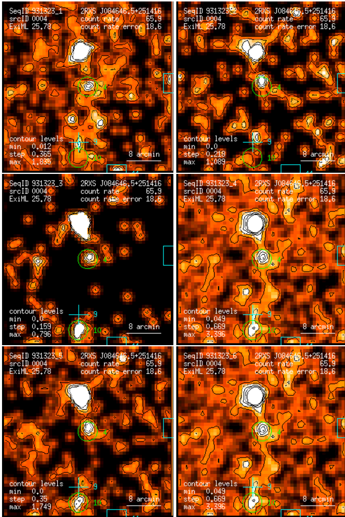
Figure 4: RASS 931323: detection 0004: band rate images, Gaussian filter: (1) PSPC channels 11 – 41, (2) 52 – 90, (3) 91 – 201, (4) 11 – 235, (5) 52 – 201, (6) 11 – 201. Broad band rates in counts/ks. Band rate contour levels in counts/ks/arcmin 2 .
