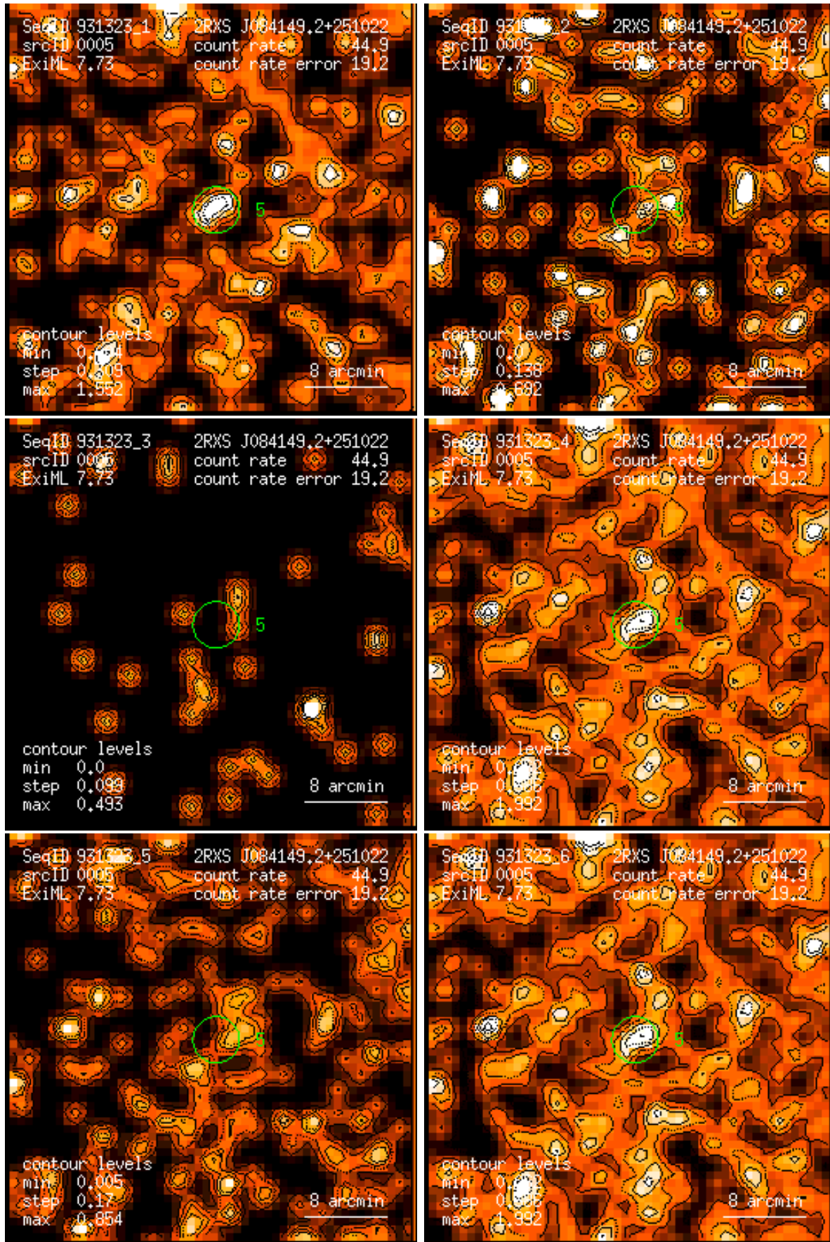
Figure 5: RASS 931323: detection 0005: band rate images, Gaussian filter: (1) PSPC channels 11 – 41, (2) 52 – 90, (3) 91 – 201, (4) 11 – 235, (5) 52 – 201, (6) 11 – 201. Broad band rates in counts/ks. Band rate contour levels in counts/ks/arcmin 2 .
