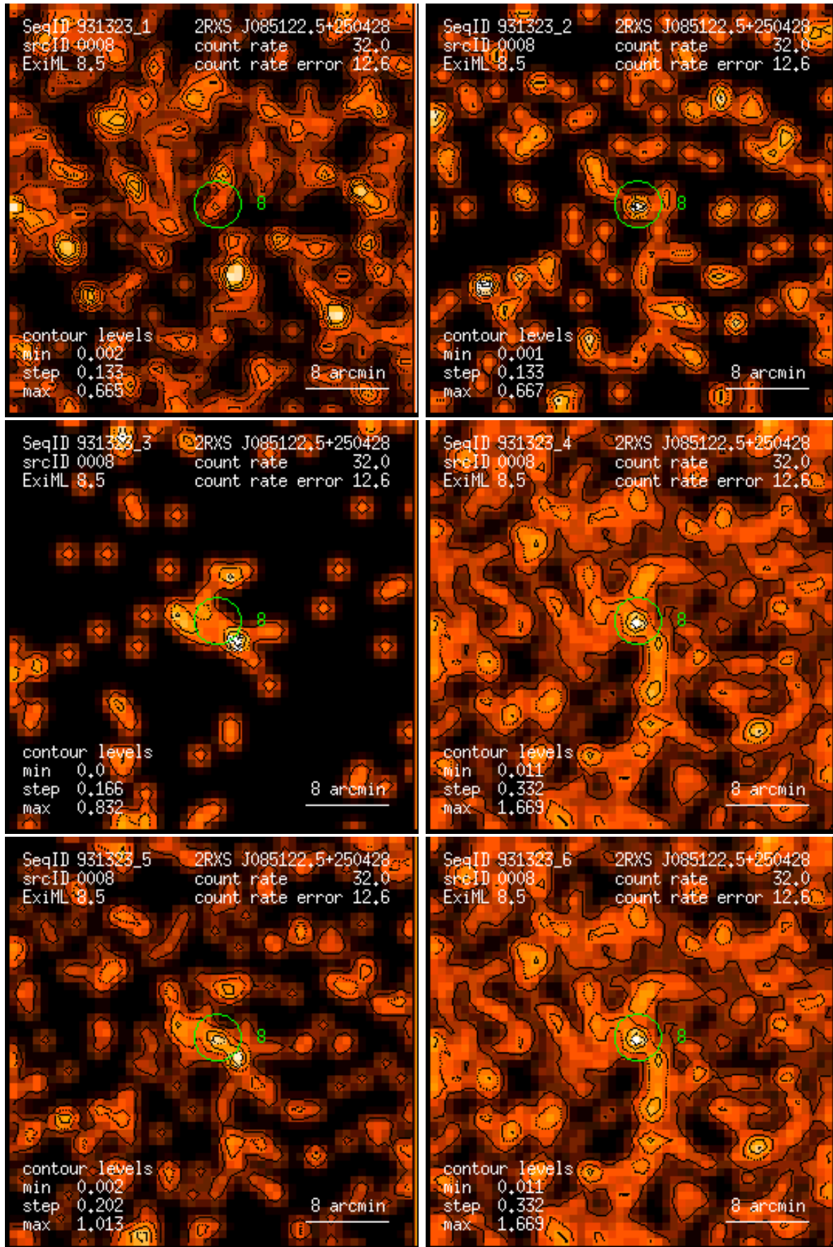
Figure 8: RASS 931323: detection 0008: band rate images, Gaussian filter: (1) PSPC channels 11 – 41, (2) 52 – 90, (3) 91 – 201, (4) 11 – 235, (5) 52 – 201, (6) 11 – 201. Broad band rates in counts/ks. Band rate contour levels in counts/ks/arcmin 2 .
