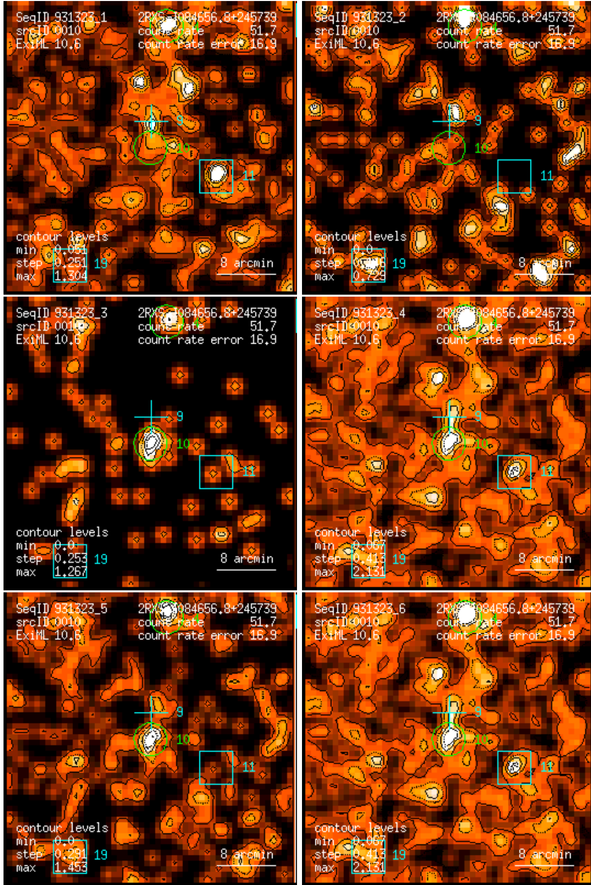
Figure 10: RASS 931323: detection 0010: band rate images, Gaussian filter: (1) PSPC channels 11 – 41, (2) 52 – 90, (3) 91 – 201, (4) 11 – 235, (5) 52 – 201, (6) 11 – 201. Broad band rates in counts/ks. Band rate contour levels in counts/ks/arcmin 2 .
