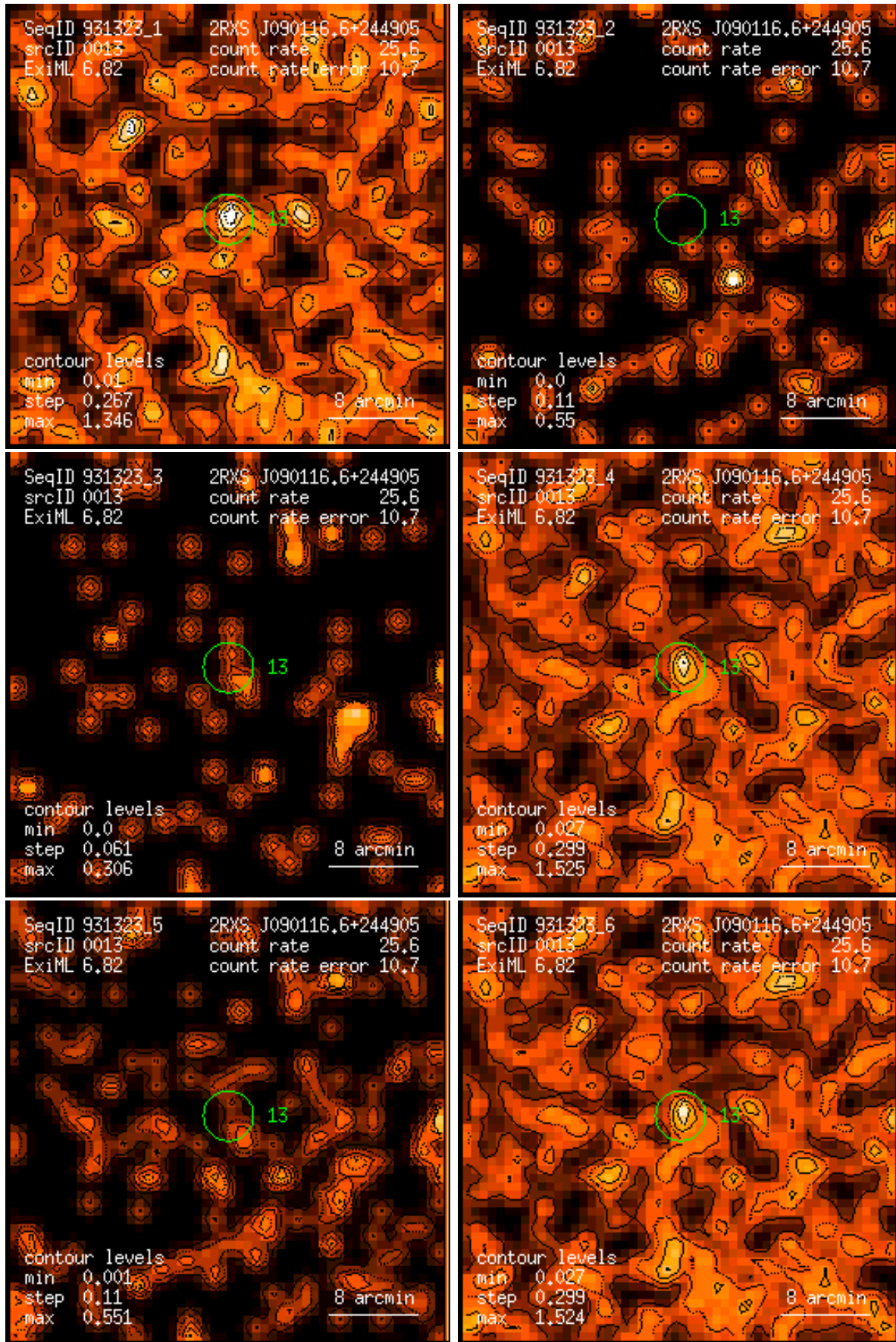
Figure 13: RASS 931323: detection 0013: band rate images, Gaussian filter: (1) PSPC channels 11 – 41, (2) 52 – 90, (3) 91 – 201, (4) 11 – 235, (5) 52 – 201, (6) 11 – 201. Broad band rates in counts/ks. Band rate contour levels in counts/ks/arcmin 2 .
