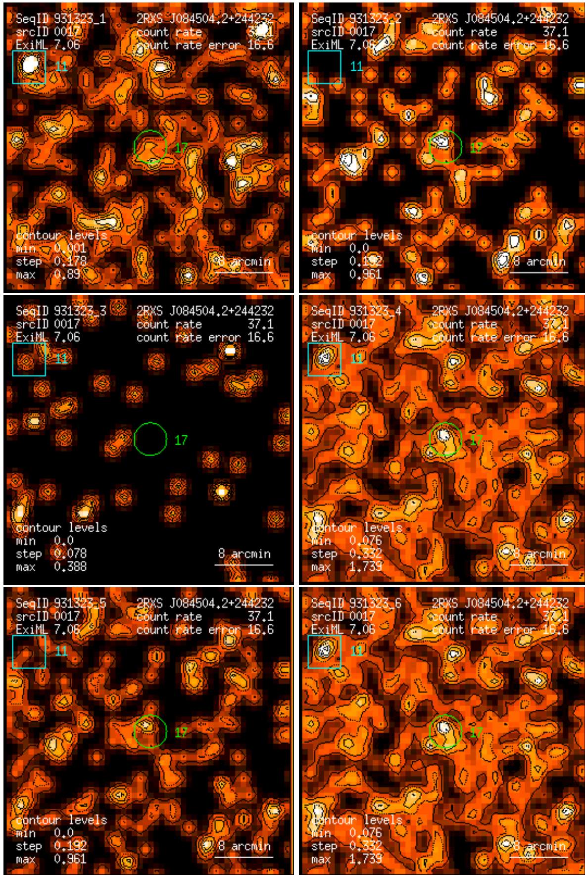
Figure 17: RASS 931323: detection 0017: band rate images, Gaussian filter: (1) PSPC channels 11 – 41, (2) 52 – 90, (3) 91 – 201, (4) 11 – 235, (5) 52 – 201, (6) 11 – 201. Broad band rates in counts/ks. Band rate contour levels in counts/ks/arcmin 2 .
