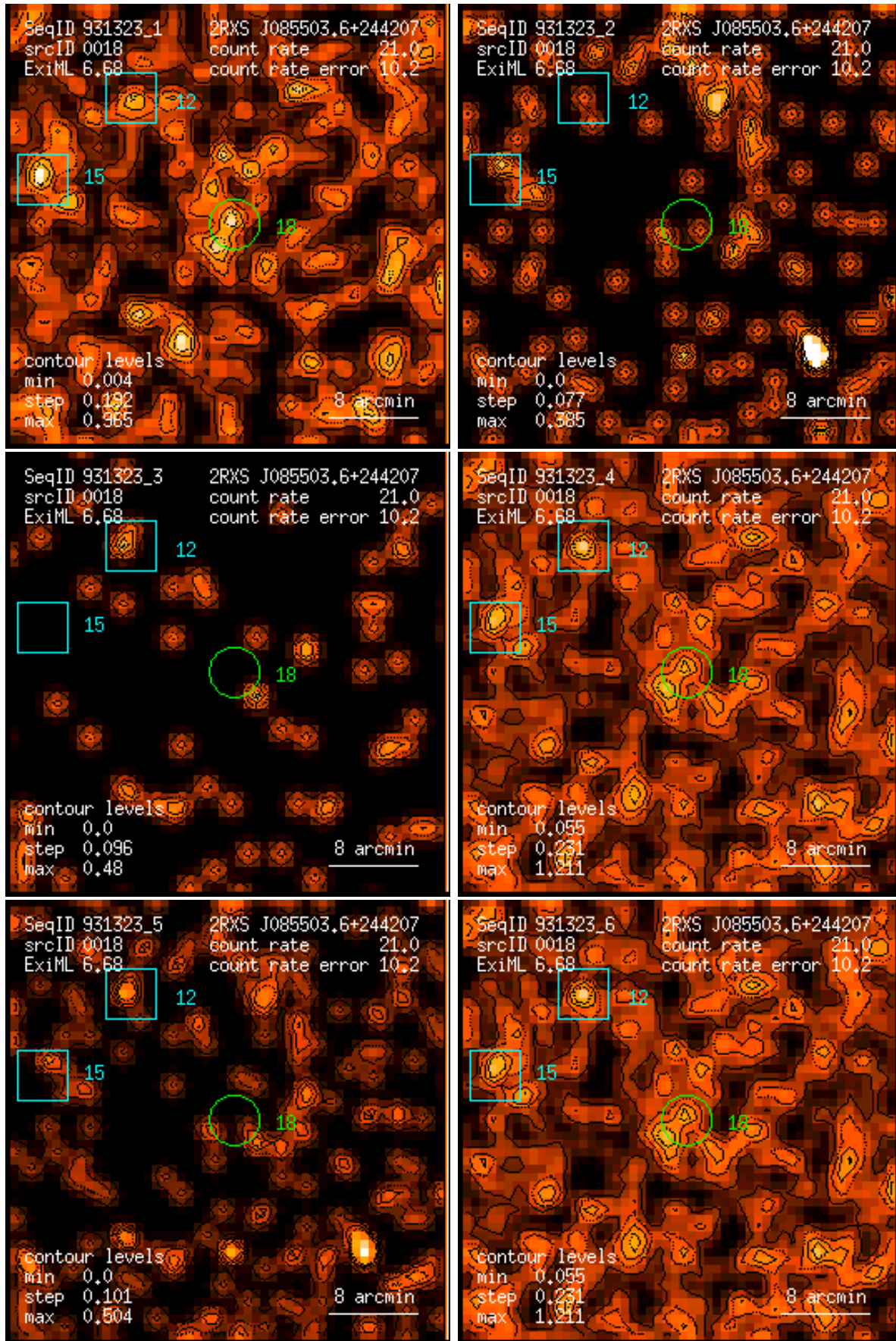
Figure 18: RASS 931323: detection 0018: band rate images, Gaussian filter: (1) PSPC channels 11 – 41, (2) 52 – 90, (3) 91 – 201, (4) 11 – 235, (5) 52 – 201, (6) 11 – 201. Broad band rates in counts/ks. Band rate contour levels in counts/ks/arcmin 2 .
