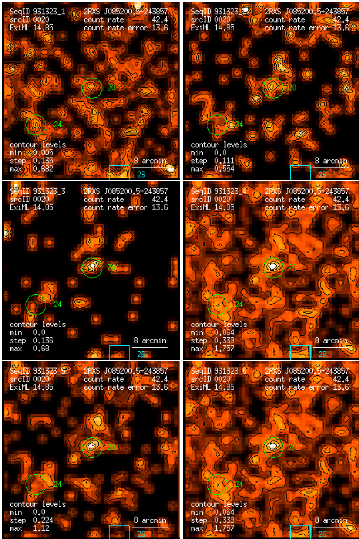
Figure 20: RASS 931323: detection 0020: band rate images, Gaussian filter: (1) PSPC channels 11 – 41, (2) 52 – 90, (3) 91 – 201, (4) 11 – 235, (5) 52 – 201, (6) 11 – 201. Broad band rates in counts/ks. Band rate contour levels in counts/ks/arcmin 2 .
