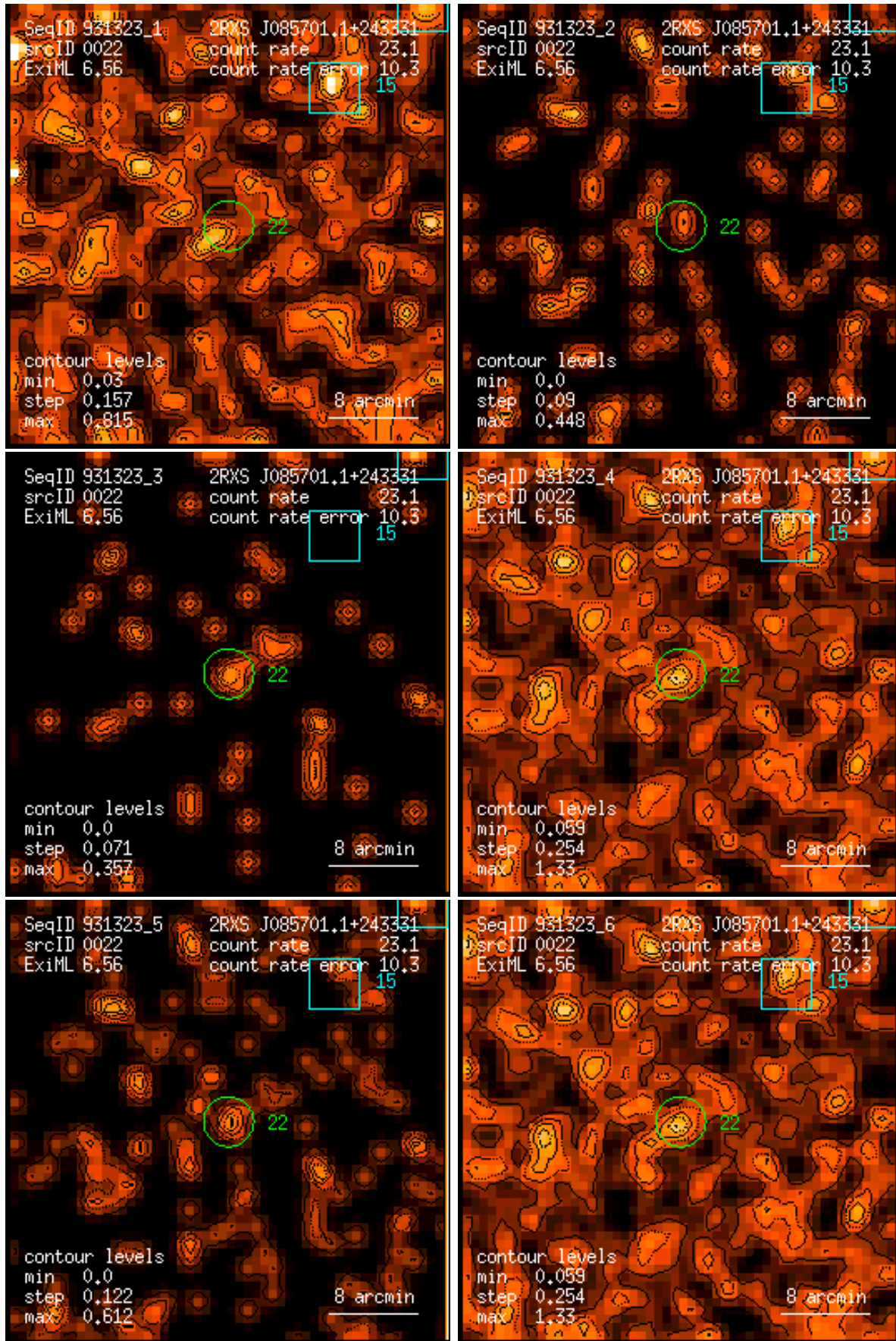
Figure 22: RASS 931323: detection 0022: band rate images, Gaussian filter: (1) PSPC channels 11 – 41, (2) 52 – 90, (3) 91 – 201, (4) 11 – 235, (5) 52 – 201, (6) 11 – 201. Broad band rates in counts/ks. Band rate contour levels in counts/ks/arcmin 2 .
