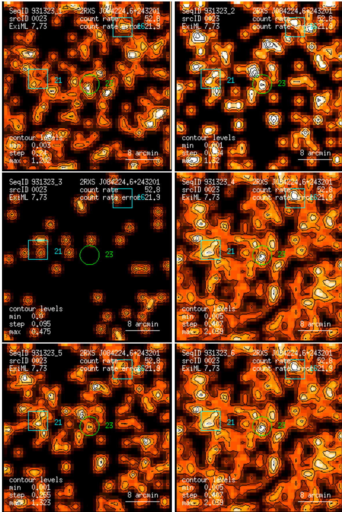
Figure 23: RASS 931323: detection 0023: band rate images, Gaussian filter: (1) PSPC channels 11 – 41, (2) 52 – 90, (3) 91 – 201, (4) 11 – 235, (5) 52 – 201, (6) 11 – 201. Broad band rates in counts/ks. Band rate contour levels in counts/ks/arcmin 2 .
