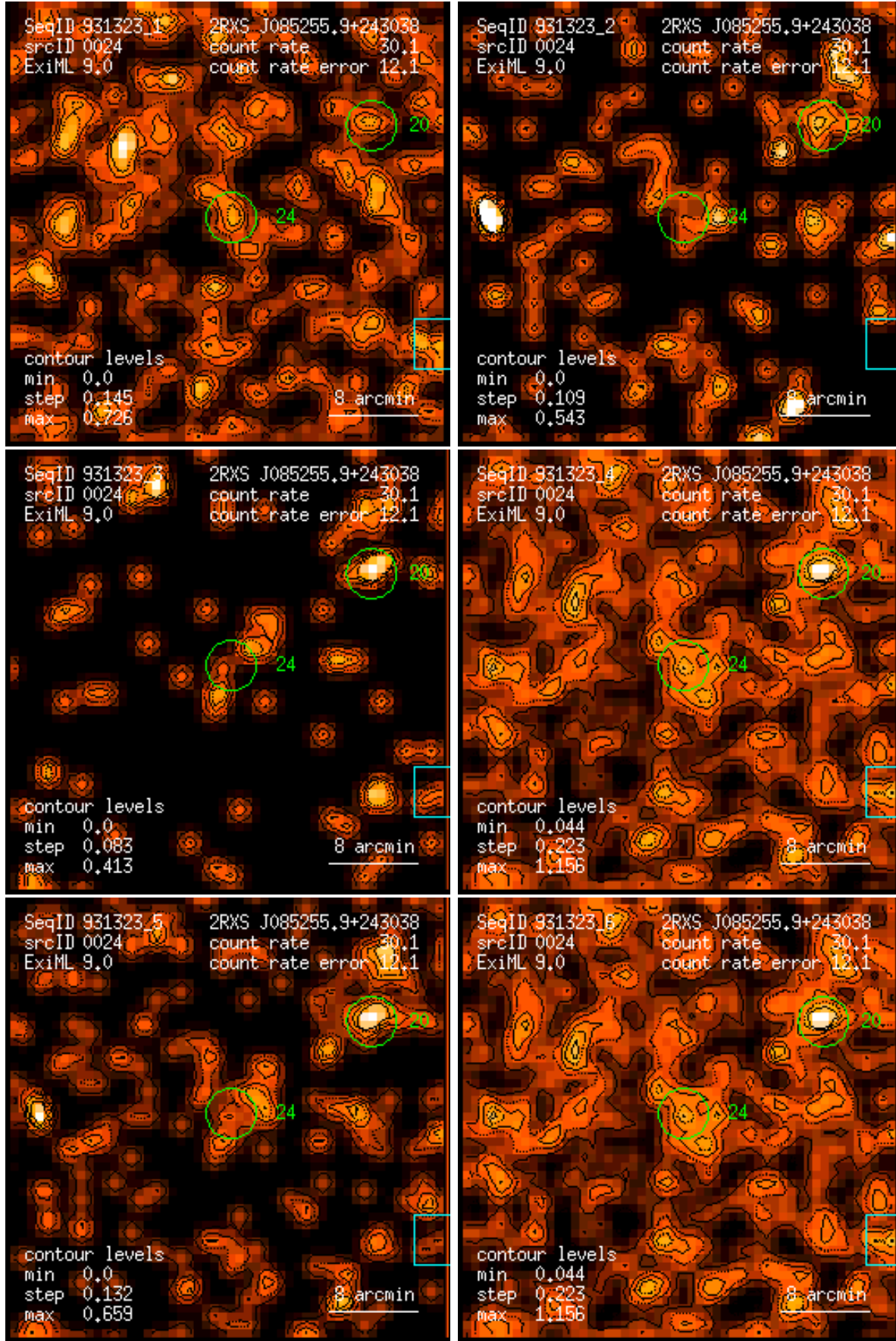
Figure 24: RASS 931323: detection 0024: band rate images, Gaussian filter: (1) PSPC channels 11 – 41, (2) 52 – 90, (3) 91 – 201, (4) 11 – 235, (5) 52 – 201, (6) 11 – 201. Broad band rates in counts/ks. Band rate contour levels in counts/ks/arcmin 2 .
