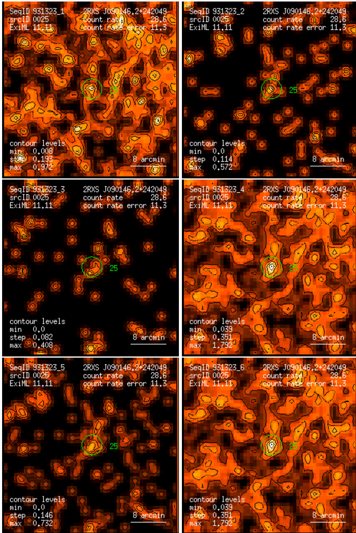
Figure 25: RASS 931323: detection 0025: band rate images, Gaussian filter: (1) PSPC channels 11 – 41, (2) 52 – 90, (3) 91 – 201, (4) 11 – 235, (5) 52 – 201, (6) 11 – 201. Broad band rates in counts/ks. Band rate contour levels in counts/ks/arcmin 2 .
