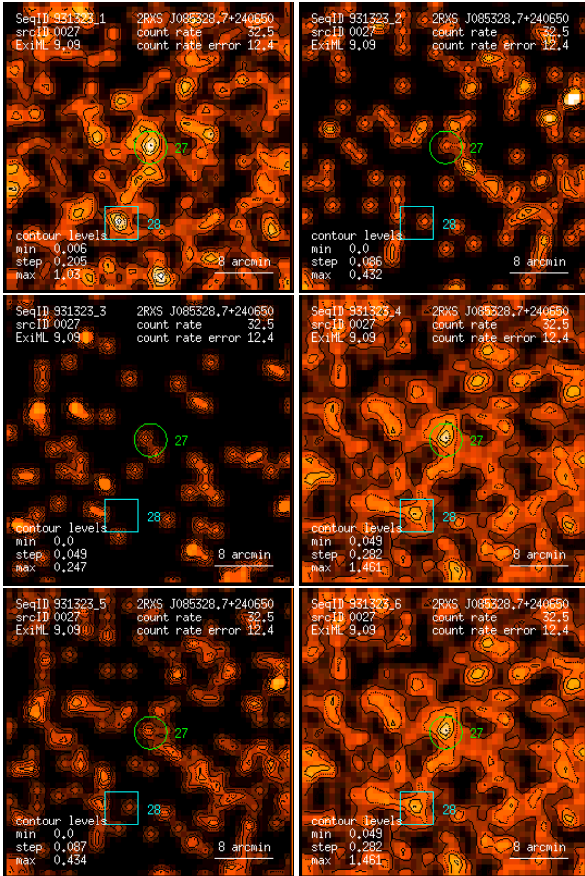
Figure 27: RASS 931323: detection 0027: band rate images, Gaussian filter: (1) PSPC channels 11 – 41, (2) 52 – 90, (3) 91 – 201, (4) 11 – 235, (5) 52 – 201, (6) 11 – 201. Broad band rates in counts/ks. Band rate contour levels in counts/ks/arcmin 2 .
