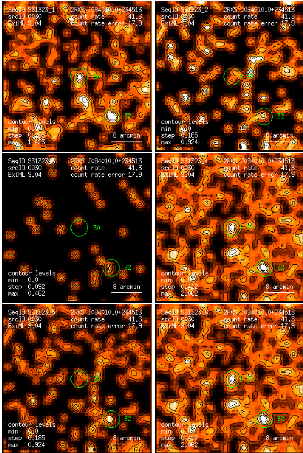
Figure 30: RASS 931323: detection 0030: band rate images, Gaussian filter: (1) PSPC channels 11 – 41, (2) 52 – 90, (3) 91 – 201, (4) 11 – 235, (5) 52 – 201, (6) 11 – 201. Broad band rates in counts/ks. Band rate contour levels in counts/ks/arcmin 2 .
