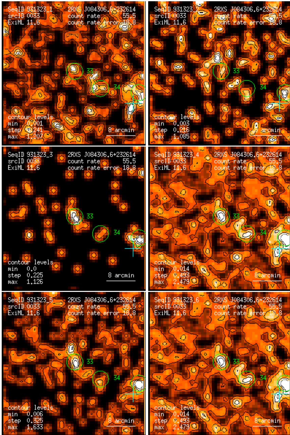
Figure 33: RASS 931323: detection 0033: band rate images, Gaussian filter: (1) PSPC channels 11 – 41, (2) 52 – 90, (3) 91 – 201, (4) 11 – 235, (5) 52 – 201, (6) 11 – 201. Broad band rates in counts/ks. Band rate contour levels in counts/ks/arcmin 2 .
