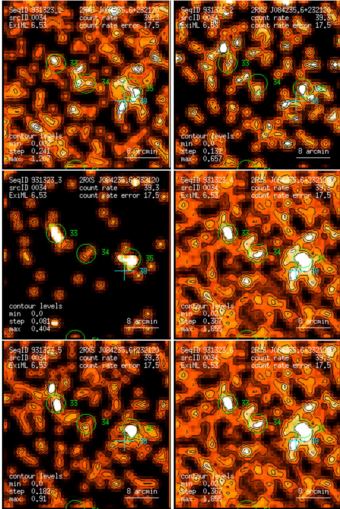
Figure 34: RASS 931323: detection 0034: band rate images, Gaussian filter: (1) PSPC channels 11 – 41, (2) 52 – 90, (3) 91 – 201, (4) 11 – 235, (5) 52 – 201, (6) 11 – 201. Broad band rates in counts/ks. Band rate contour levels in counts/ks/arcmin 2 .
