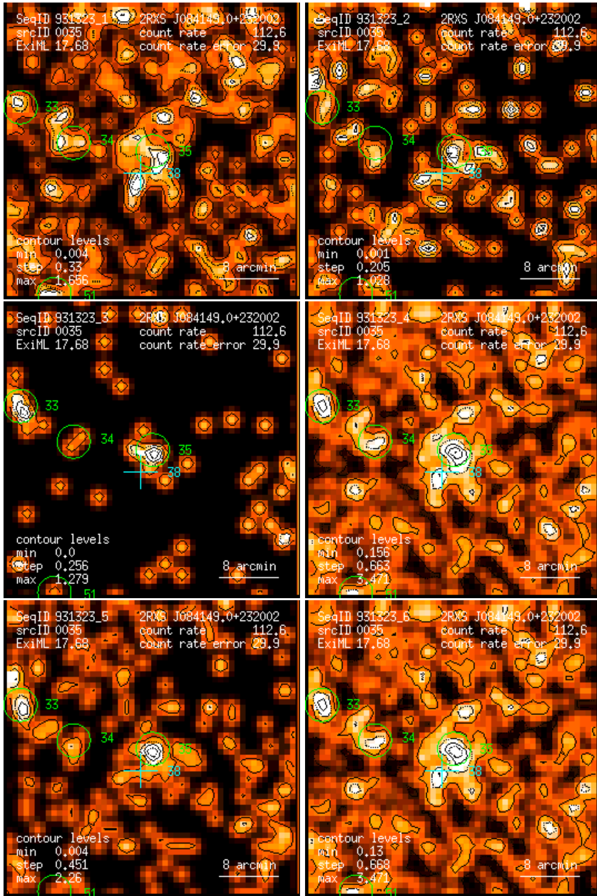
Figure 35: RASS 931323: detection 0035: band rate images, Gaussian filter: (1) PSPC channels 11 – 41, (2) 52 – 90, (3) 91 – 201, (4) 11 – 235, (5) 52 – 201, (6) 11 – 201. Broad band rates in counts/ks. Band rate contour levels in counts/ks/arcmin 2 .
