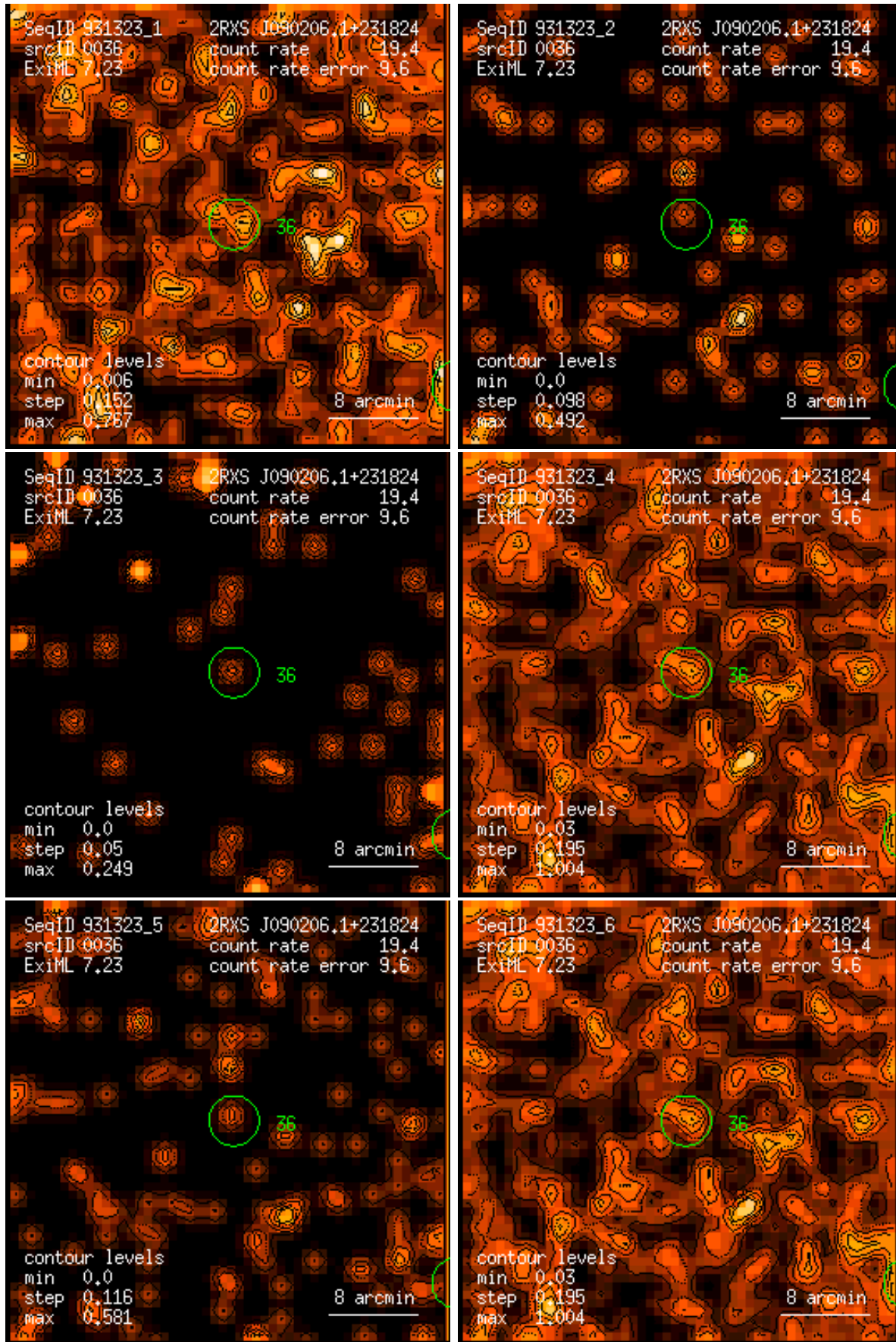
Figure 36: RASS 931323: detection 0036: band rate images, Gaussian filter: (1) PSPC channels 11 – 41, (2) 52 – 90, (3) 91 – 201, (4) 11 – 235, (5) 52 – 201, (6) 11 – 201. Broad band rates in counts/ks. Band rate contour levels in counts/ks/arcmin 2 .
