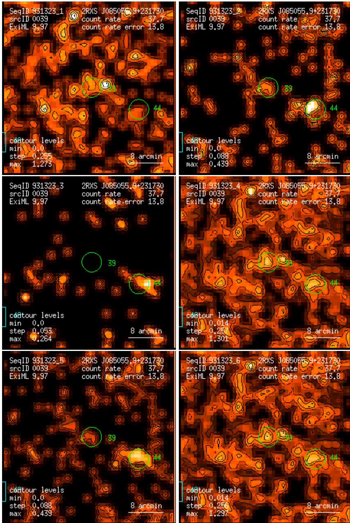
Figure 39: RASS 931323: detection 0039: band rate images, Gaussian filter: (1) PSPC channels 11 – 41, (2) 52 – 90, (3) 91 – 201, (4) 11 – 235, (5) 52 – 201, (6) 11 – 201. Broad band rates in counts/ks. Band rate contour levels in counts/ks/arcmin 2 .
