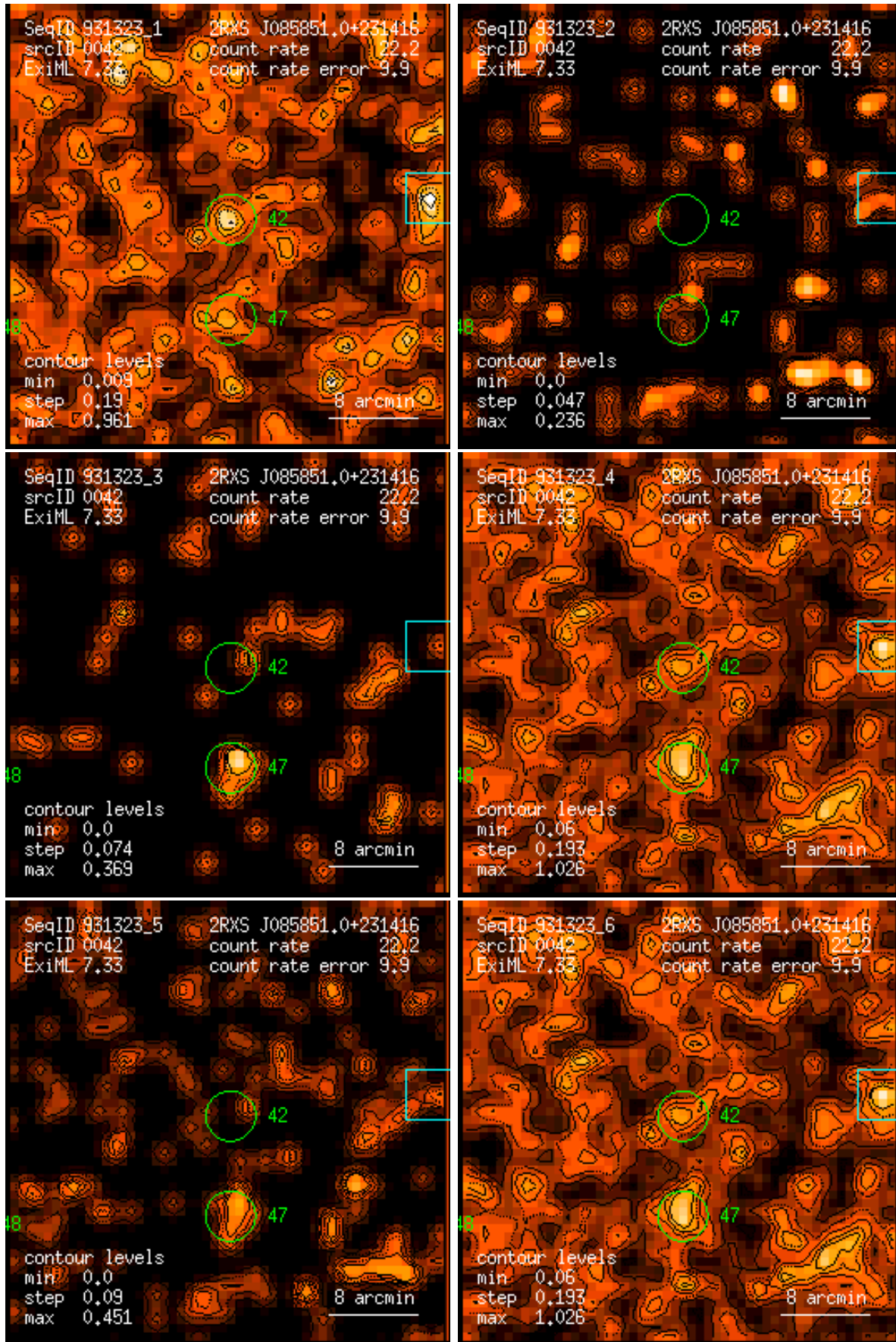
Figure 42: RASS 931323: detection 0042: band rate images, Gaussian filter: (1) PSPC channels 11 – 41, (2) 52 – 90, (3) 91 – 201, (4) 11 – 235, (5) 52 – 201, (6) 11 – 201. Broad band rates in counts/ks. Band rate contour levels in counts/ks/arcmin 2 .
