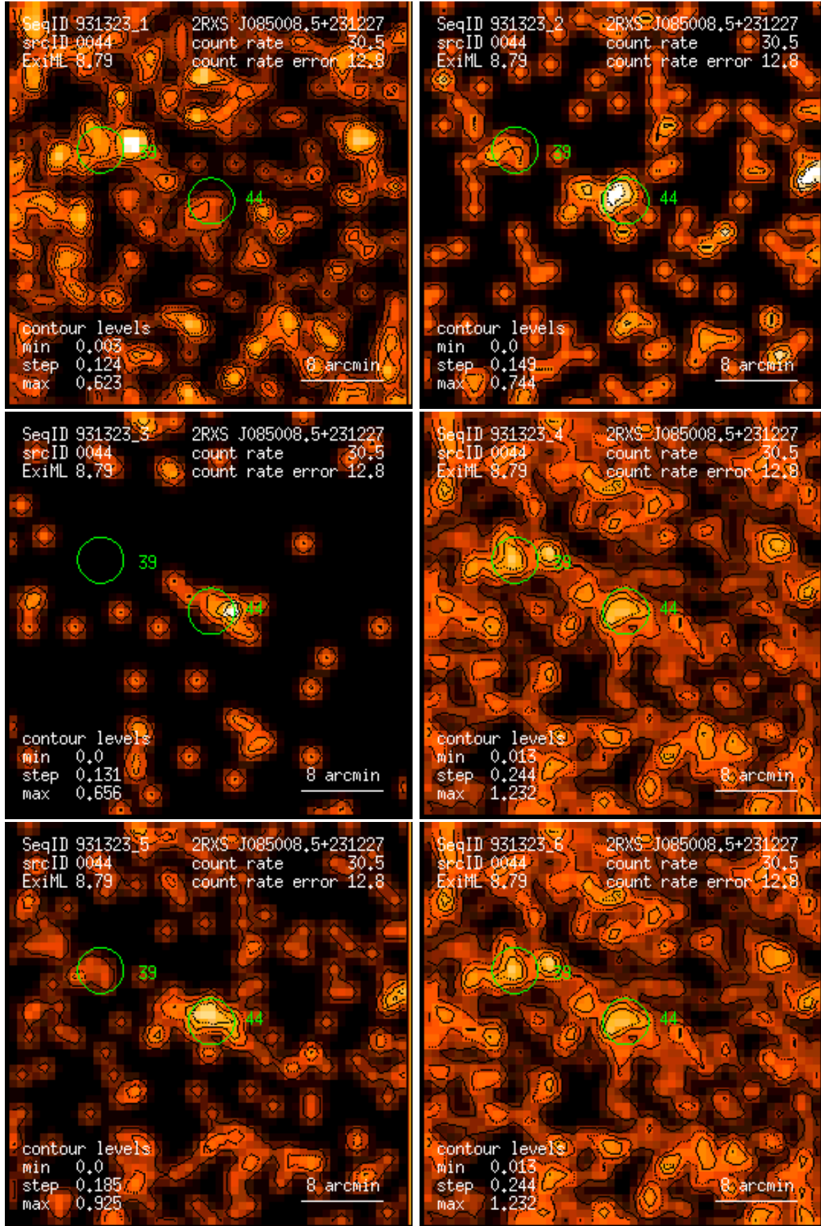
Figure 44: RASS 931323: detection 0044: band rate images, Gaussian filter: (1) PSPC channels 11 – 41, (2) 52 – 90, (3) 91 – 201, (4) 11 – 235, (5) 52 – 201, (6) 11 – 201. Broad band rates in counts/ks. Band rate contour levels in counts/ks/arcmin 2 .
