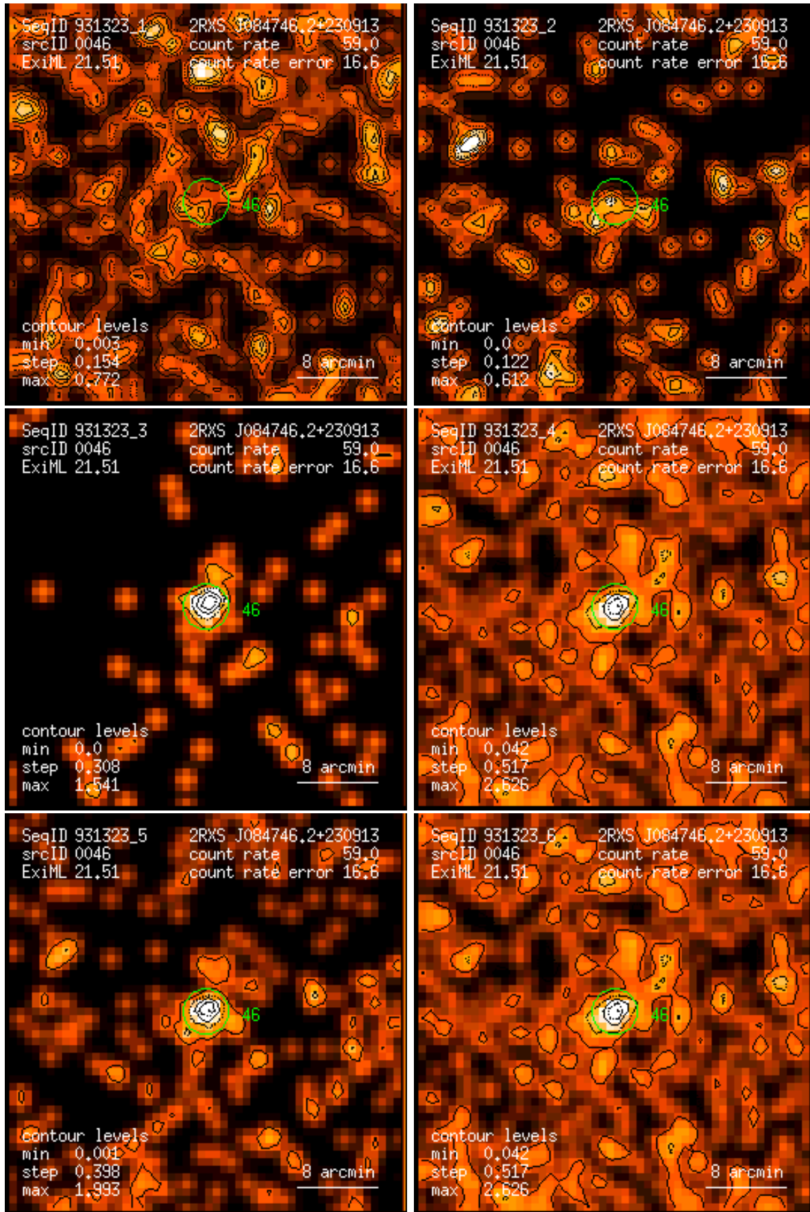
Figure 46: RASS 931323: detection 0046: band rate images, Gaussian filter: (1) PSPC channels 11 – 41, (2) 52 – 90, (3) 91 – 201, (4) 11 – 235, (5) 52 – 201, (6) 11 – 201. Broad band rates in counts/ks. Band rate contour levels in counts/ks/arcmin 2 .
