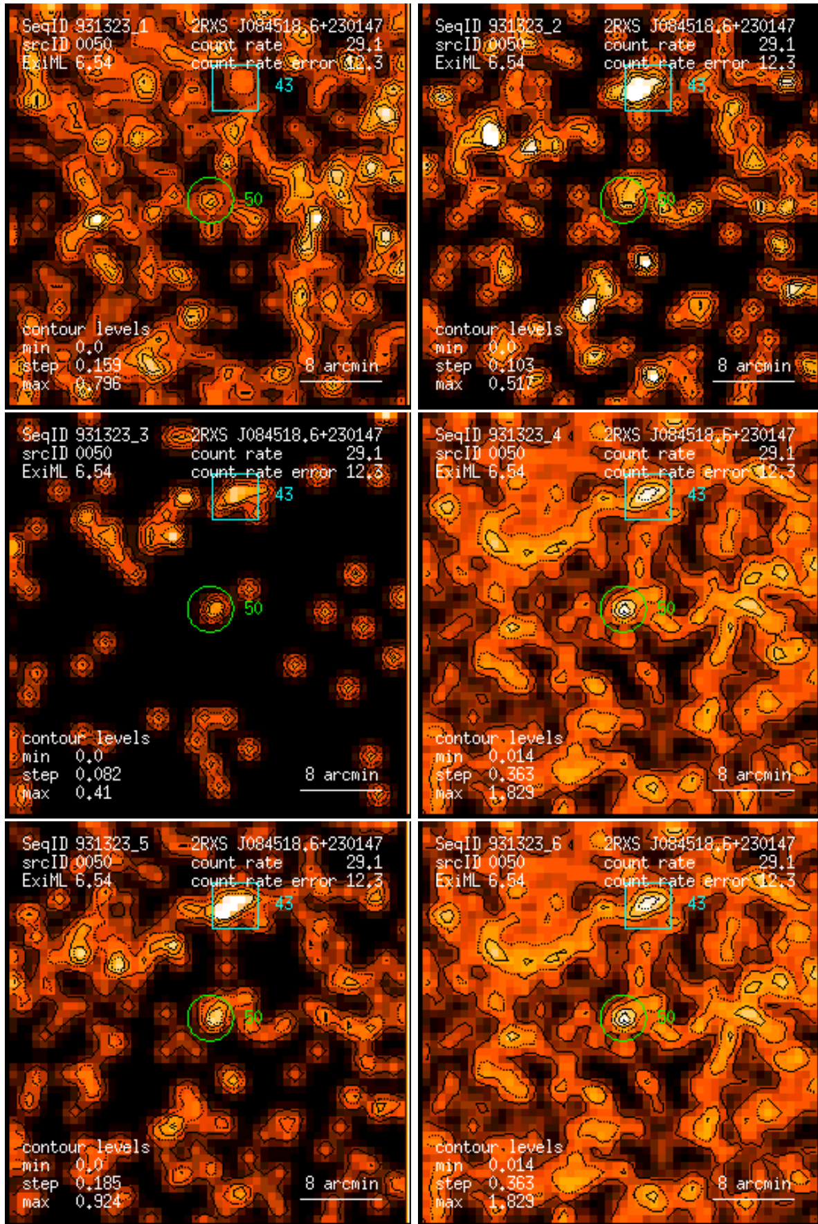
Figure 50: RASS 931323: detection 0050: band rate images, Gaussian filter: (1) PSPC channels 11 – 41, (2) 52 – 90, (3) 91 – 201, (4) 11 – 235, (5) 52 – 201, (6) 11 – 201. Broad band rates in counts/ks. Band rate contour levels in counts/ks/arcmin 2 .
