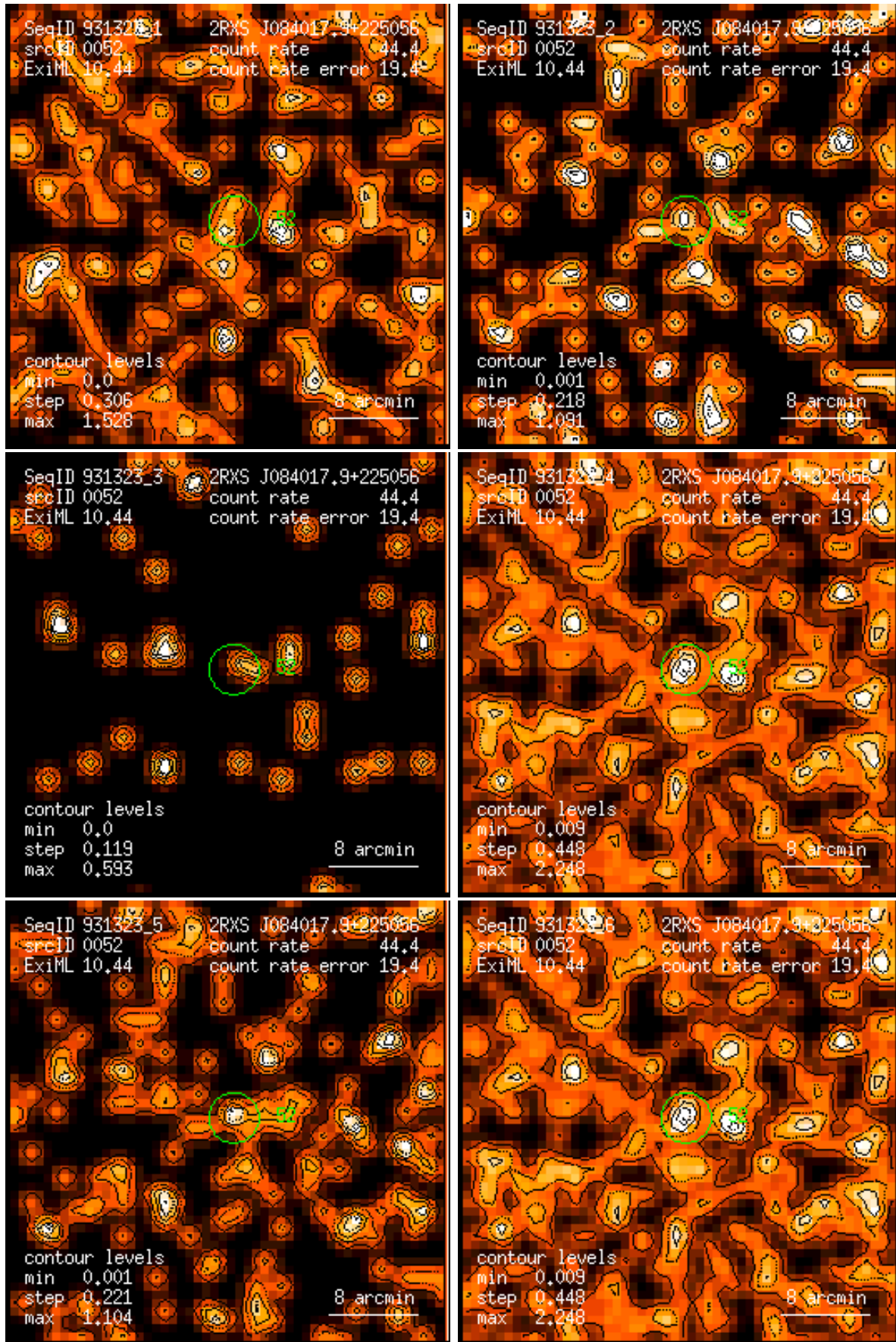
Figure 52: RASS 931323: detection 0052: band rate images, Gaussian filter: (1) PSPC channels 11 – 41, (2) 52 – 90, (3) 91 – 201, (4) 11 – 235, (5) 52 – 201, (6) 11 – 201. Broad band rates in counts/ks. Band rate contour levels in counts/ks/arcmin 2 .
