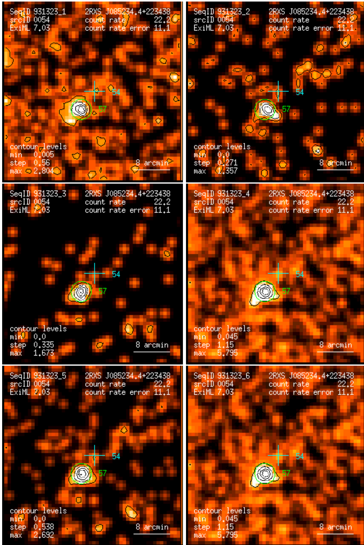
Figure 54: RASS 931323: detection 0054: band rate images, Gaussian filter: (1) PSPC channels 11 – 41, (2) 52 – 90, (3) 91 – 201, (4) 11 – 235, (5) 52 – 201, (6) 11 – 201. Broad band rates in counts/ks. Band rate contour levels in counts/ks/arcmin 2 .
