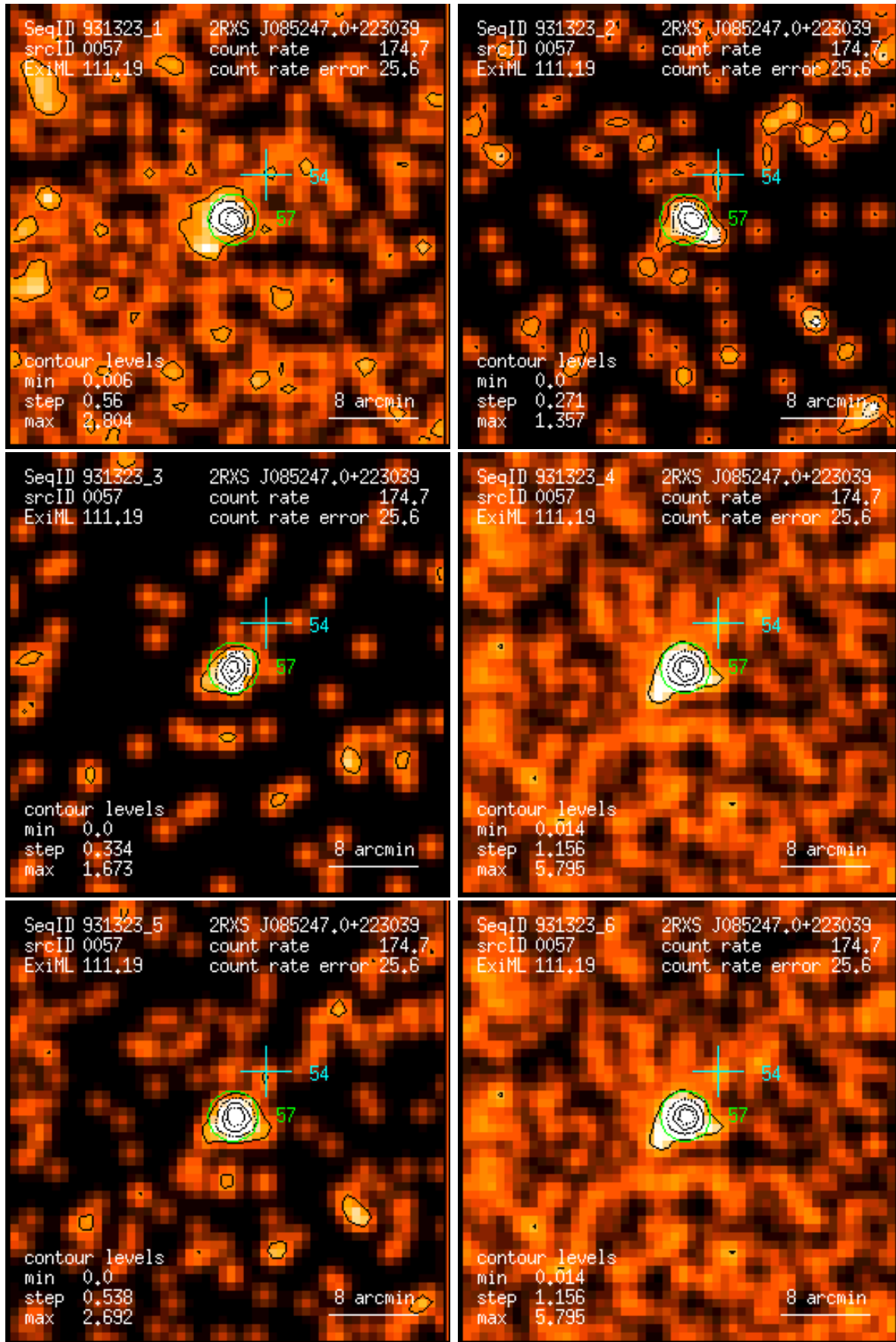
Figure 57: RASS 931323: detection 0057: band rate images, Gaussian filter: (1) PSPC channels 11 – 41, (2) 52 – 90, (3) 91 – 201, (4) 11 – 235, (5) 52 – 201, (6) 11 – 201. Broad band rates in counts/ks. Band rate contour levels in counts/ks/arcmin 2 .
