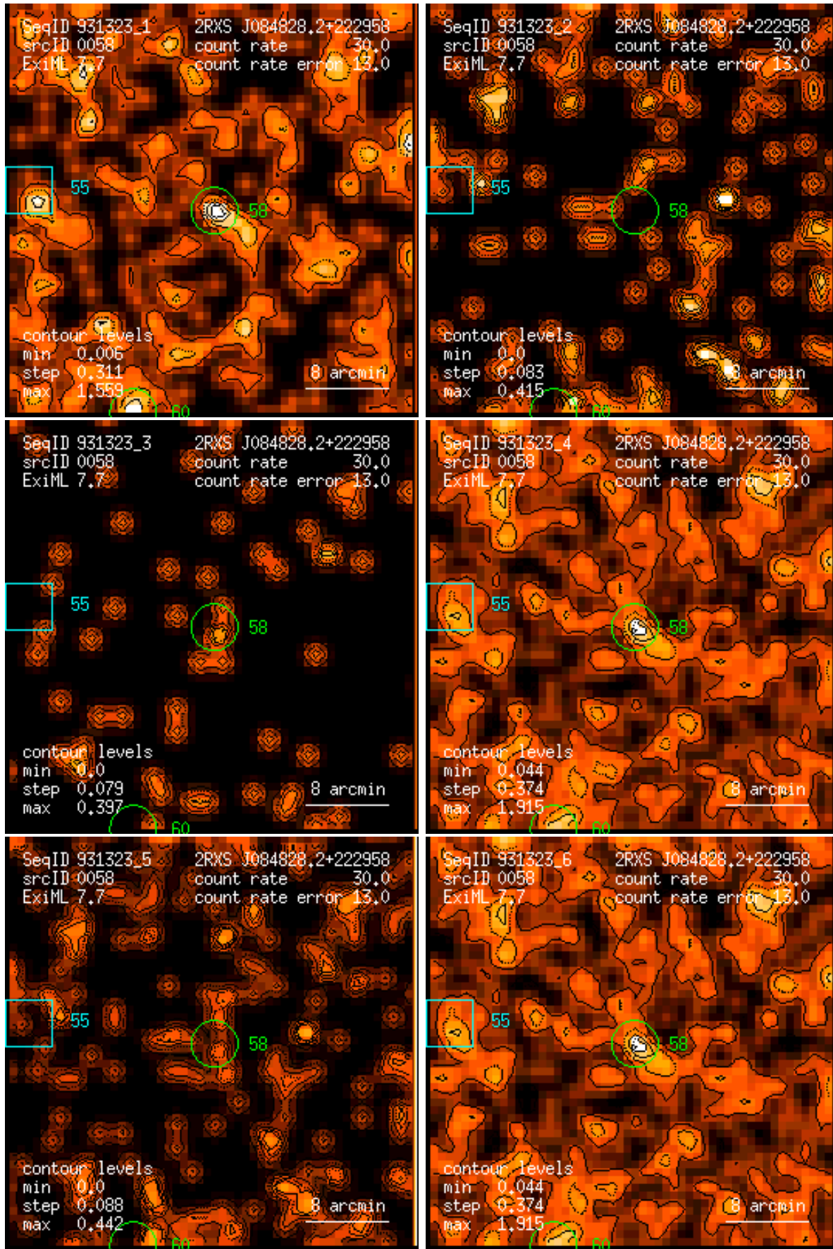
Figure 58: RASS 931323: detection 0058: band rate images, Gaussian filter: (1) PSPC channels 11 – 41, (2) 52 – 90, (3) 91 – 201, (4) 11 – 235, (5) 52 – 201, (6) 11 – 201. Broad band rates in counts/ks. Band rate contour levels in counts/ks/arcmin 2 .
