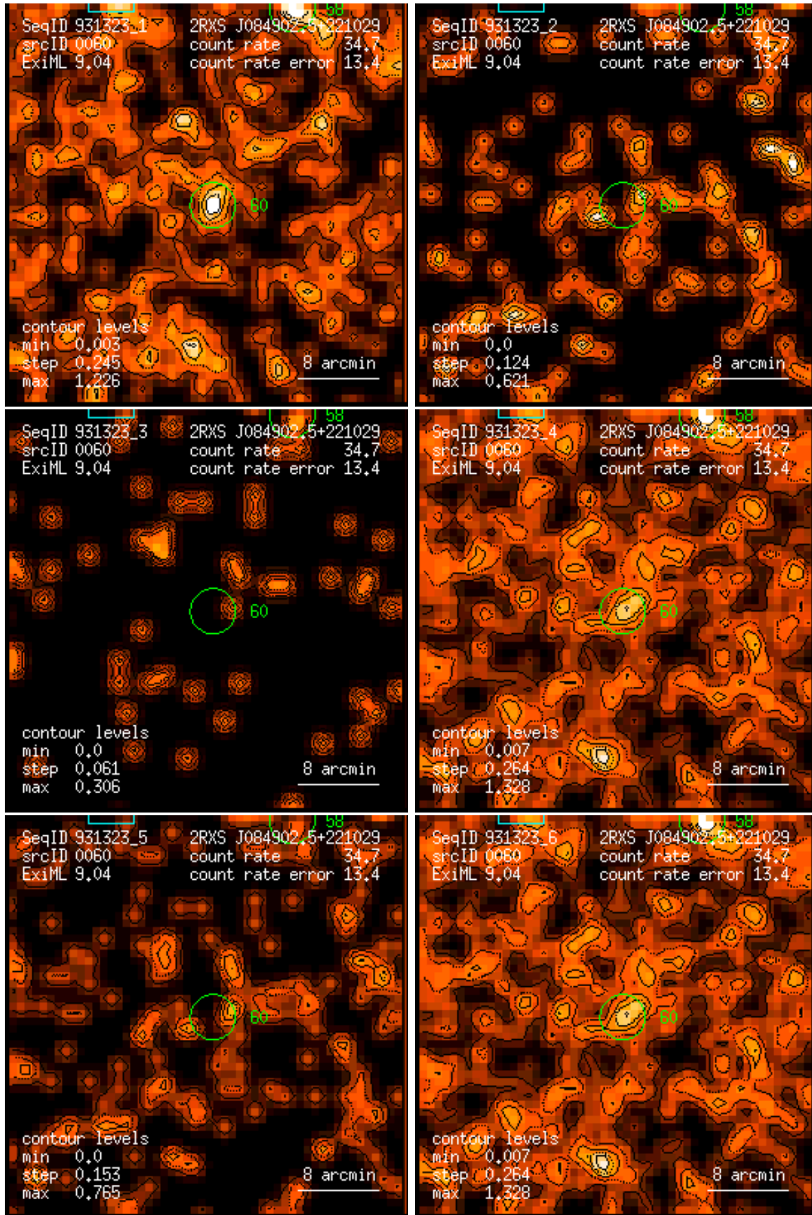
Figure 60: RASS 931323: detection 0060: band rate images, Gaussian filter: (1) PSPC channels 11 – 41, (2) 52 – 90, (3) 91 – 201, (4) 11 – 235, (5) 52 – 201, (6) 11 – 201. Broad band rates in counts/ks. Band rate contour levels in counts/ks/arcmin 2 .
