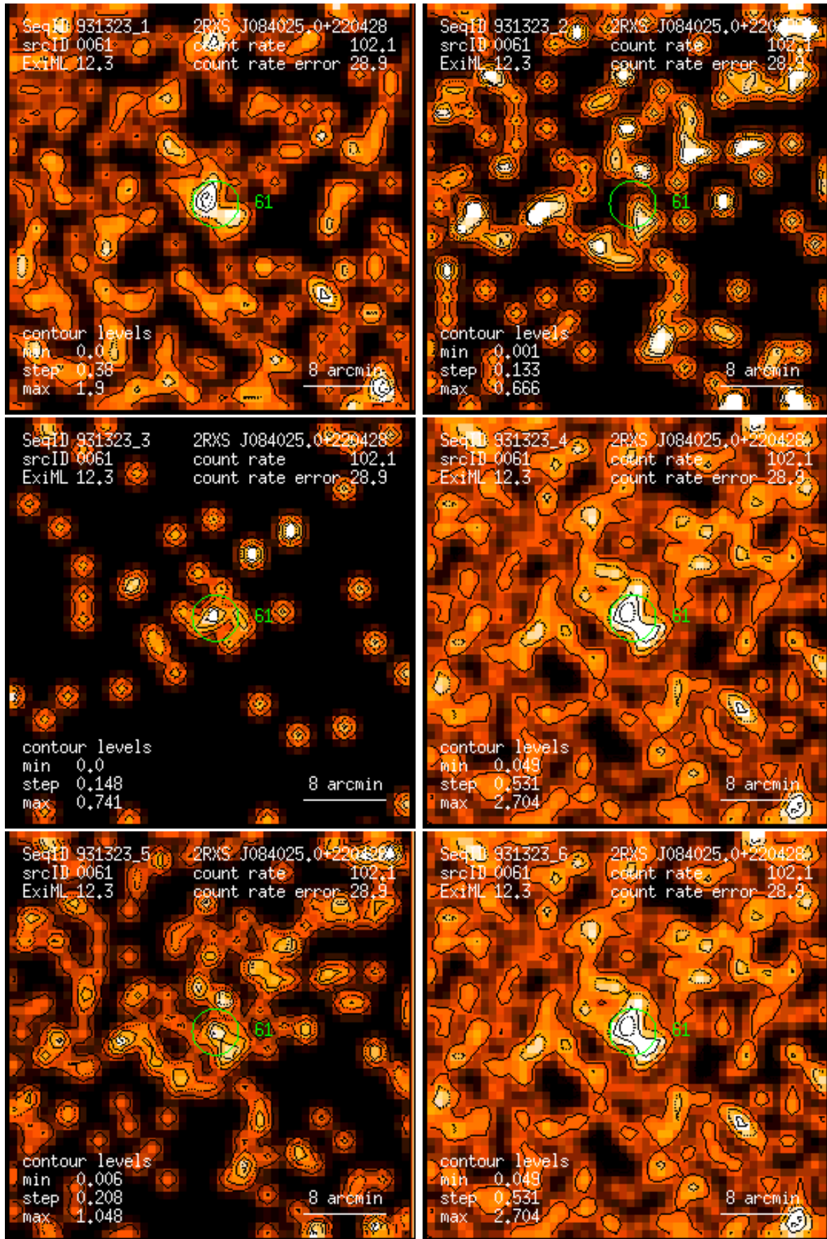
Figure 61: RASS 931323: detection 0061: band rate images, Gaussian filter: (1) PSPC channels 11 – 41, (2) 52 – 90, (3) 91 – 201, (4) 11 – 235, (5) 52 – 201, (6) 11 – 201. Broad band rates in counts/ks. Band rate contour levels in counts/ks/arcmin 2 .
