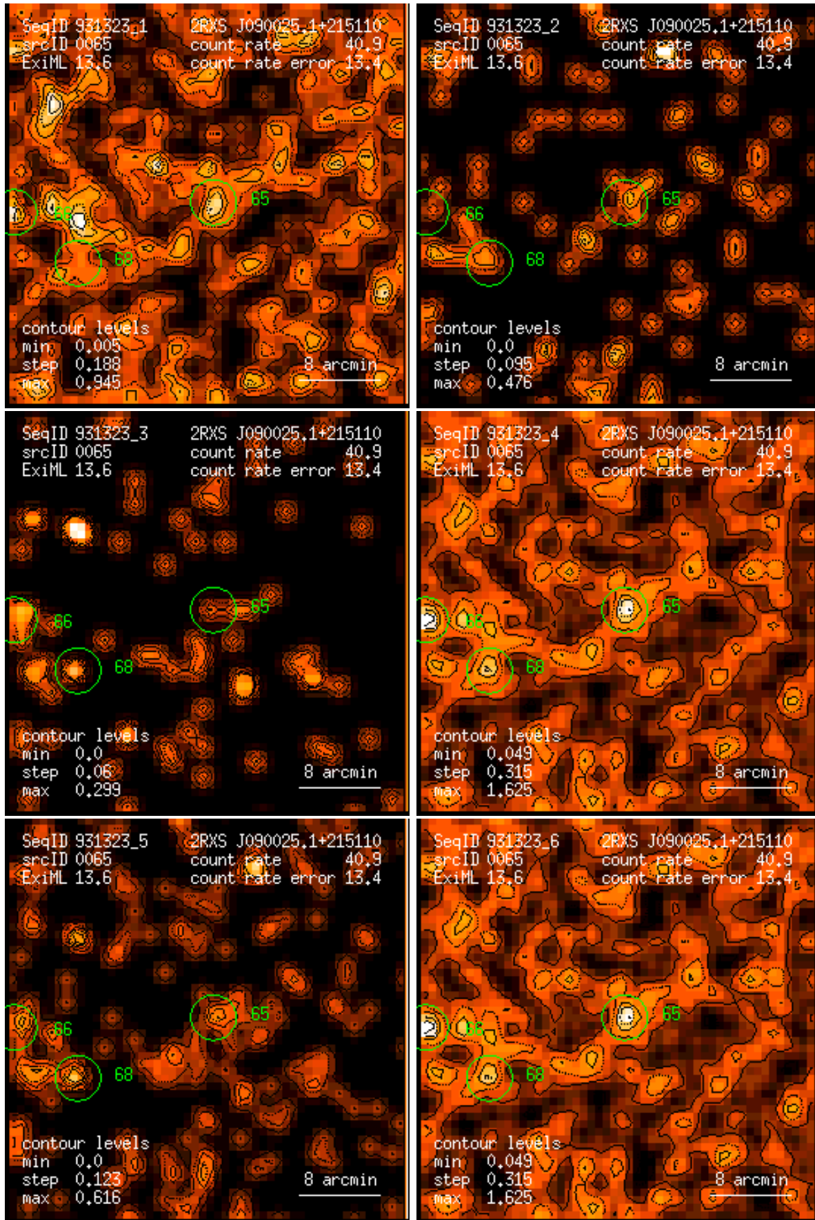
Figure 65: RASS 931323: detection 0065: band rate images, Gaussian filter: (1) PSPC channels 11 – 41, (2) 52 – 90, (3) 91 – 201, (4) 11 – 235, (5) 52 – 201, (6) 11 – 201. Broad band rates in counts/ks. Band rate contour levels in counts/ks/arcmin 2 .
