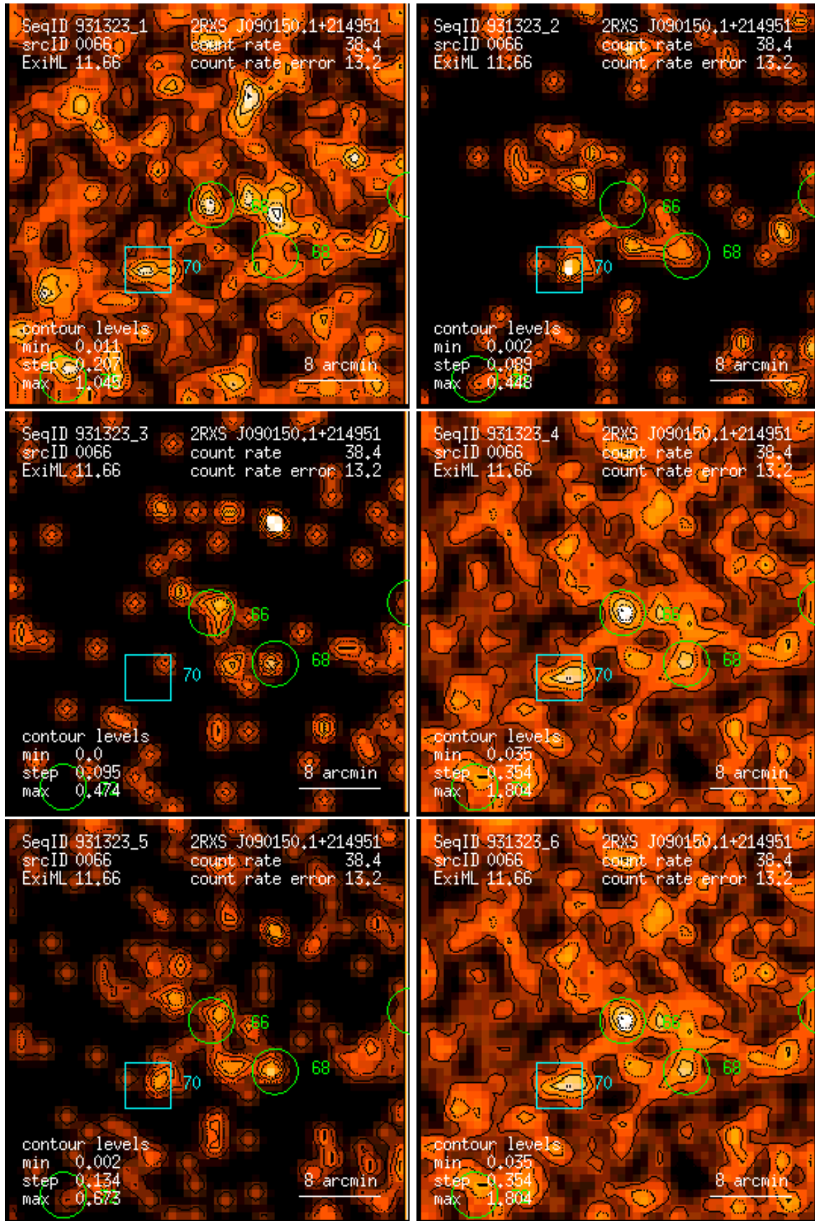
Figure 66: RASS 931323: detection 0066: band rate images, Gaussian filter: (1) PSPC channels 11 – 41, (2) 52 – 90, (3) 91 – 201, (4) 11 – 235, (5) 52 – 201, (6) 11 – 201. Broad band rates in counts/ks. Band rate contour levels in counts/ks/arcmin 2 .
