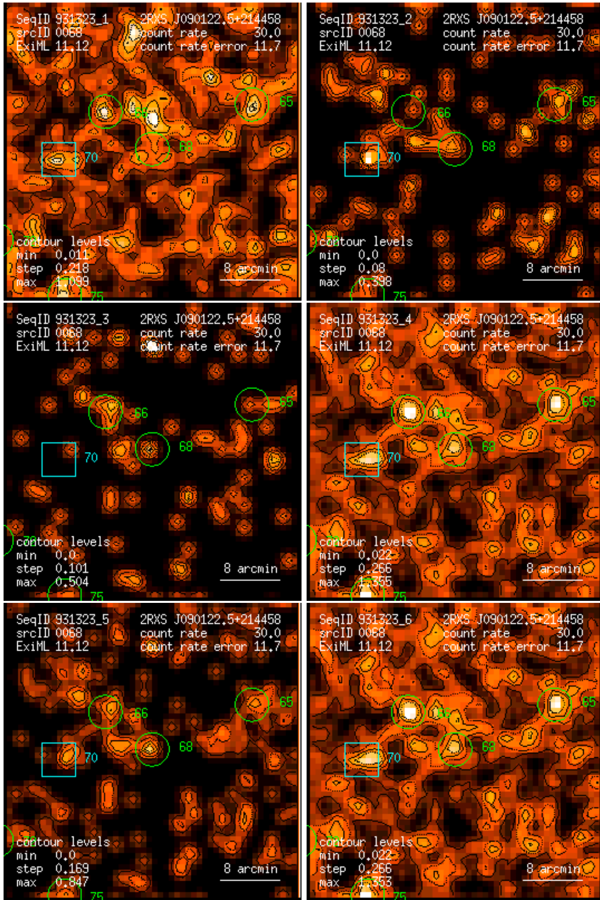
Figure 68: RASS 931323: detection 0068: band rate images, Gaussian filter: (1) PSPC channels 11 – 41, (2) 52 – 90, (3) 91 – 201, (4) 11 – 235, (5) 52 – 201, (6) 11 – 201. Broad band rates in counts/ks. Band rate contour levels in counts/ks/arcmin 2 .
