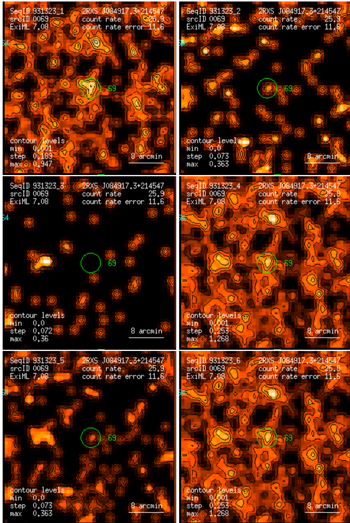
Figure 69: RASS 931323: detection 0069: band rate images, Gaussian filter: (1) PSPC channels 11 – 41, (2) 52 – 90, (3) 91 – 201, (4) 11 – 235, (5) 52 – 201, (6) 11 – 201. Broad band rates in counts/ks. Band rate contour levels in counts/ks/arcmin 2 .
